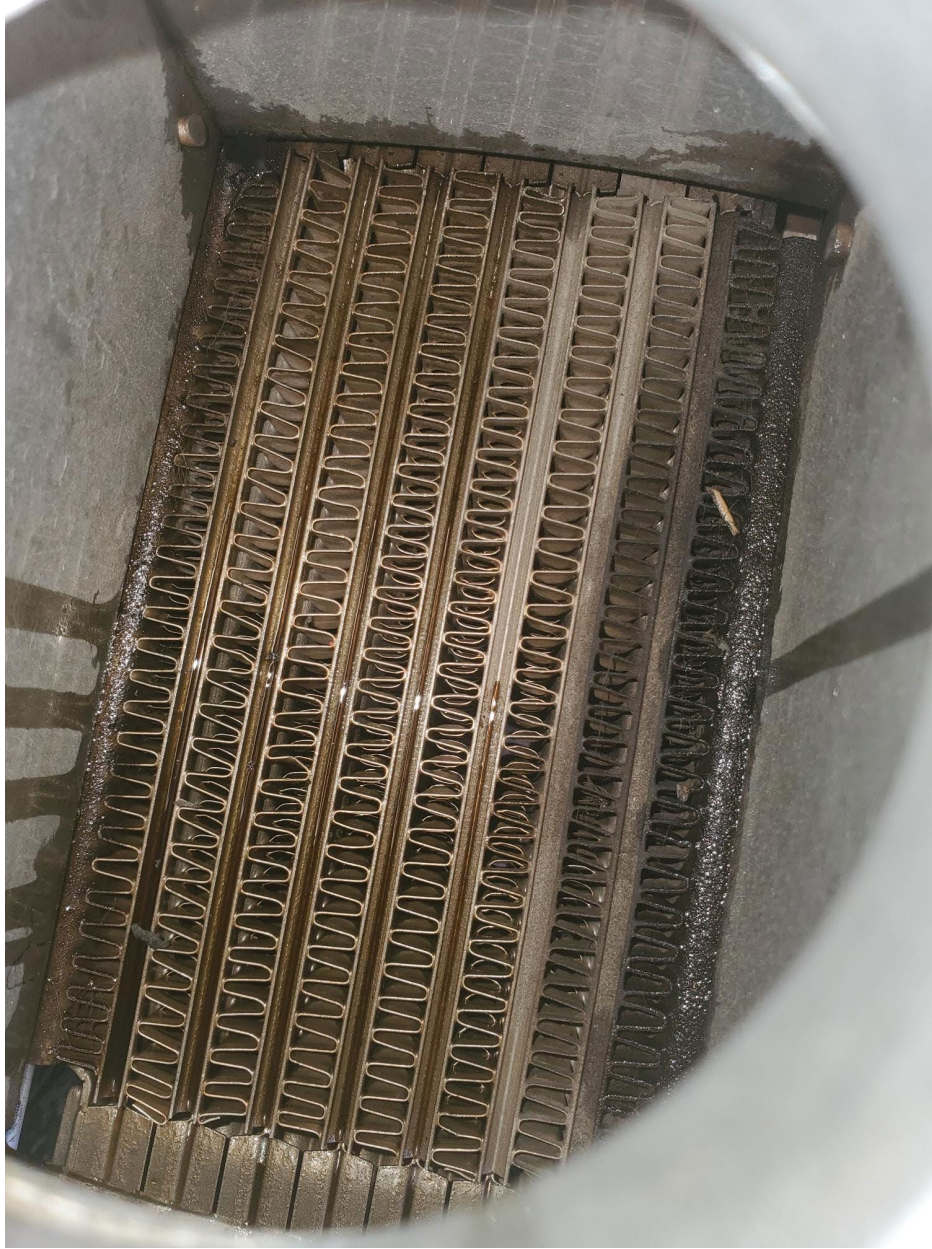
Photo 3: Engine Oil Cooler (Source – Federal Aviation Administration)
