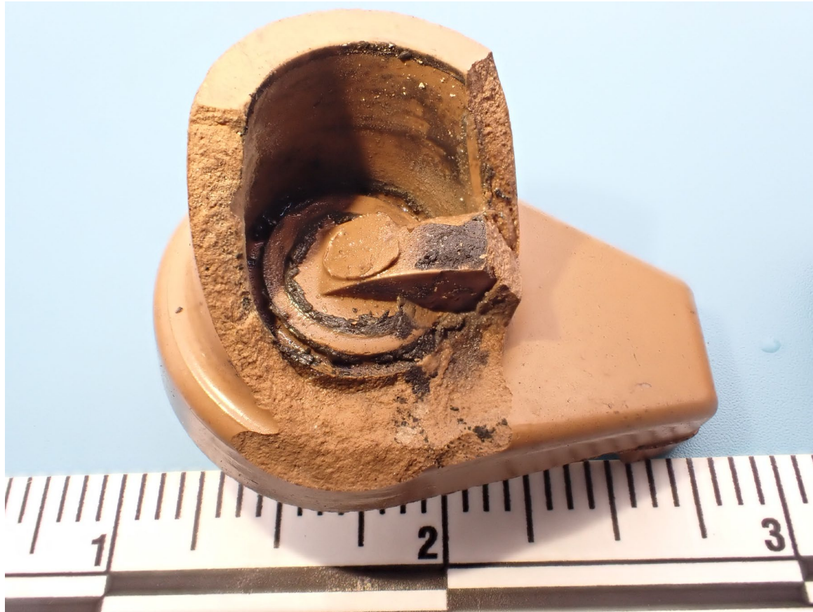
Photograph 4 - Ignition distributor rotor (NTSB Photo)
