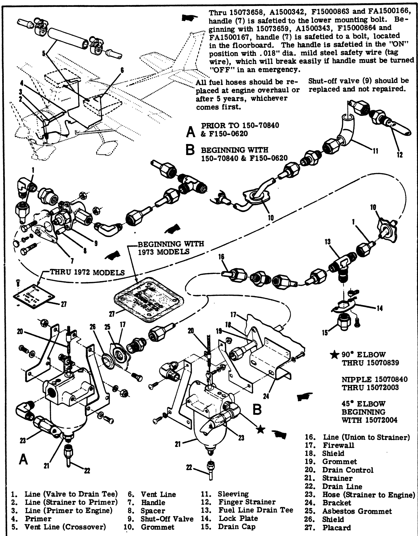
Figure 12-2. Fuel System
