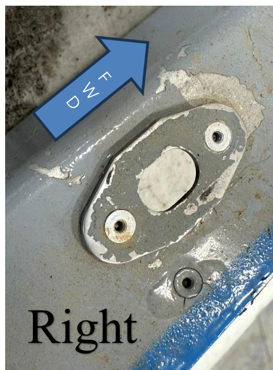
Photograph 5 - Canopy Side Pin Guides (Courtesy of Van's Aircraft)
