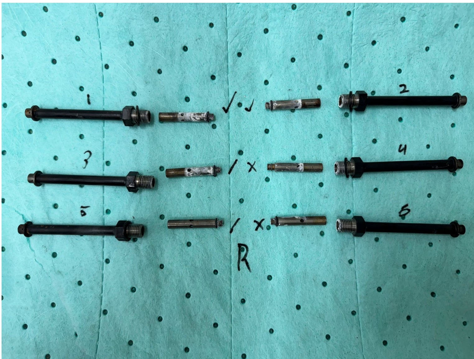
Photograph 11 - Right Engine Fuel Injectors - X Indicates Full Blockage - / Indicates Partial
