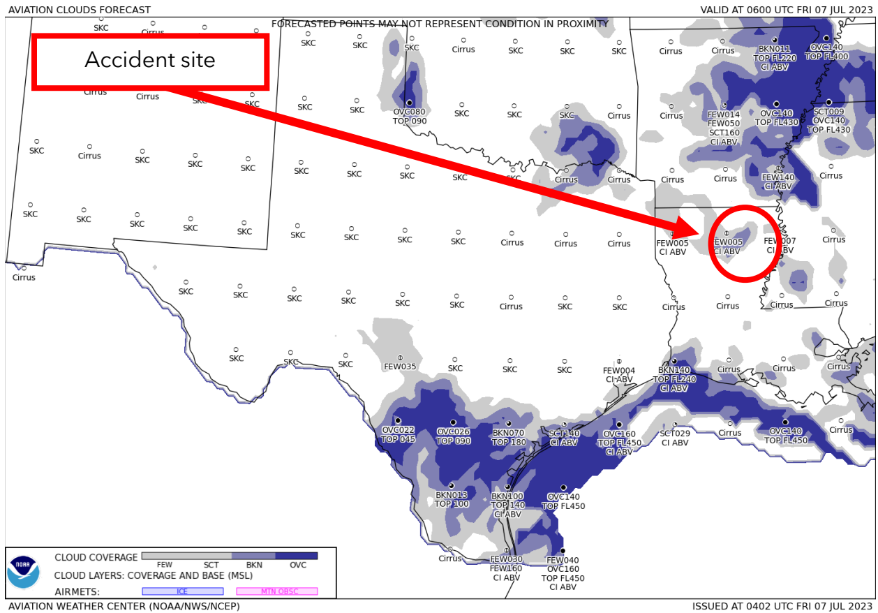
Figure 6. GFA Aviation Clouds Forecast valid at 0100 CDT with forecast issued at 2302 CDT on July 6.
