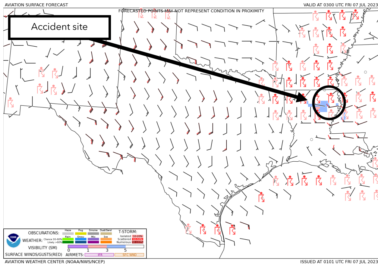
Figure 1. GFA Surface Forecast valid at 2200 CDT on July 6 with forecast issued at 2001 CDT on July 6.
