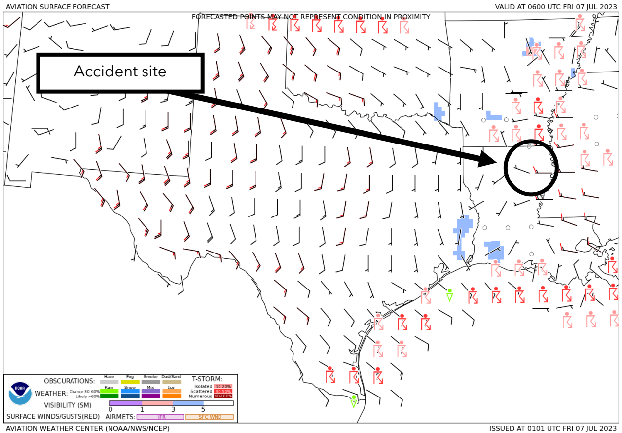
Figure 2. GFA Surface Forecast valid at 0100 CDT with forecast issued at 2001 CDT on July 6.
