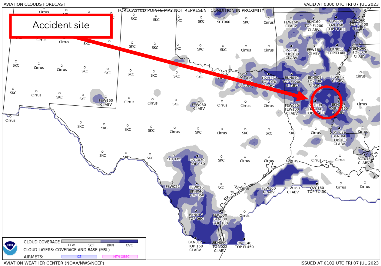
Figure 4. GFA Aviation Clouds Forecast valid at 2200 CDT on July 6 with forecast issued at 2002 CDT on July 6.
