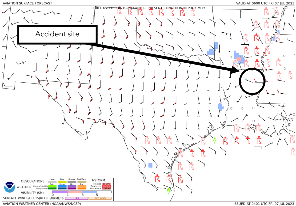
Figure 3. GFA Surface Forecast valid at 0100 CDT with forecast issued at 2301 CDT on July 6.
