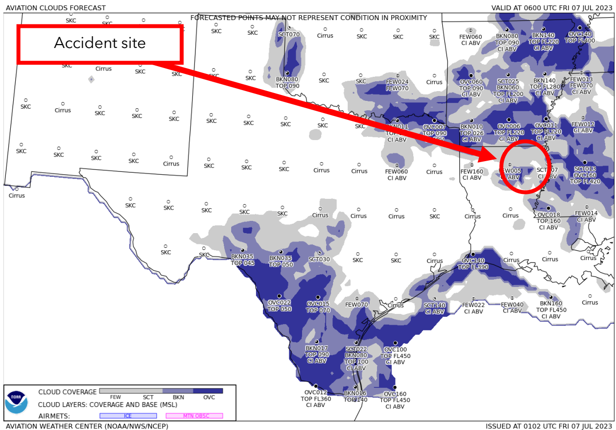
Figure 5. GFA Aviation Clouds Forecast valid at 0100 CDT with forecast issued at 2002 CDT on July 6.
