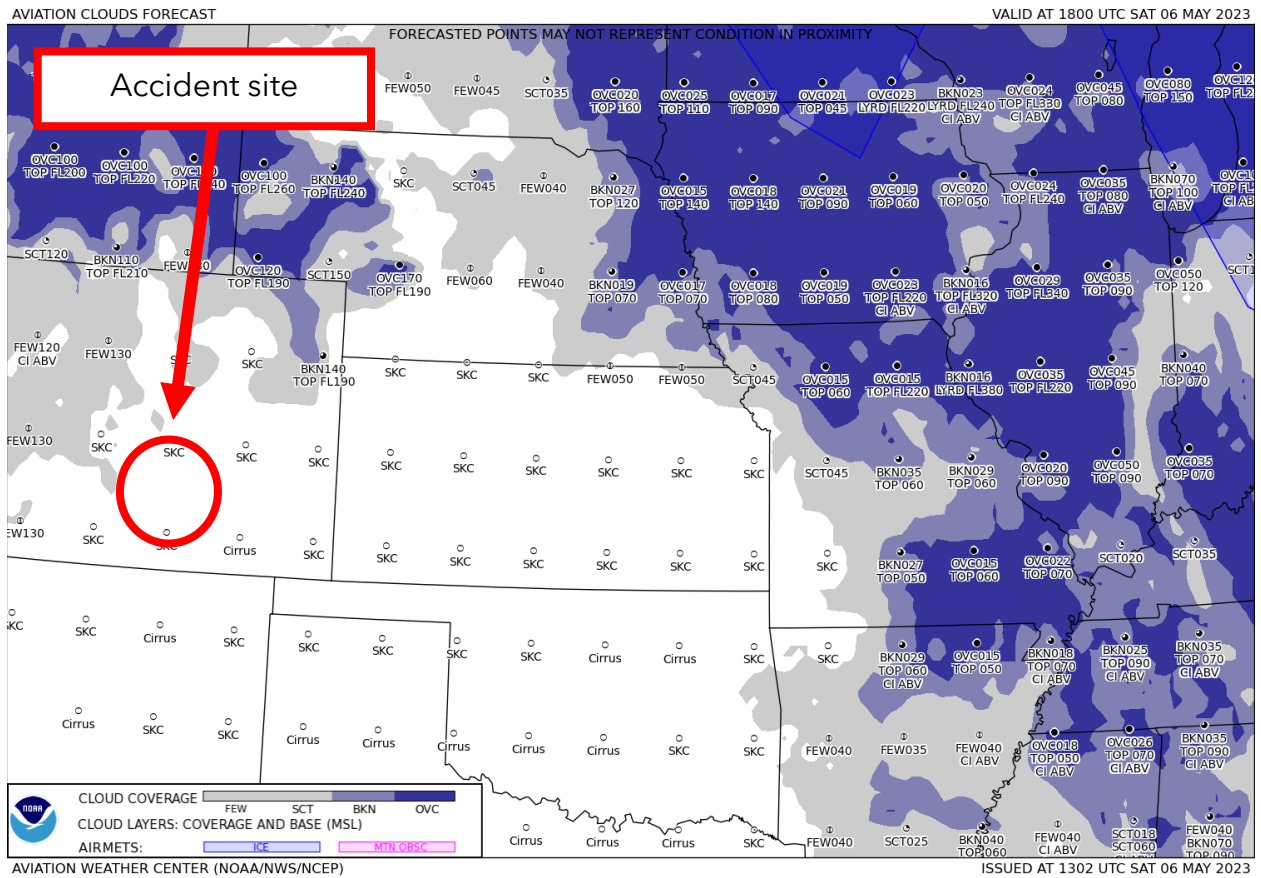
Figure 5. GFA Aviation Clouds Forecast valid at 1200 MDT with forecast issued at 0702 MDT.
