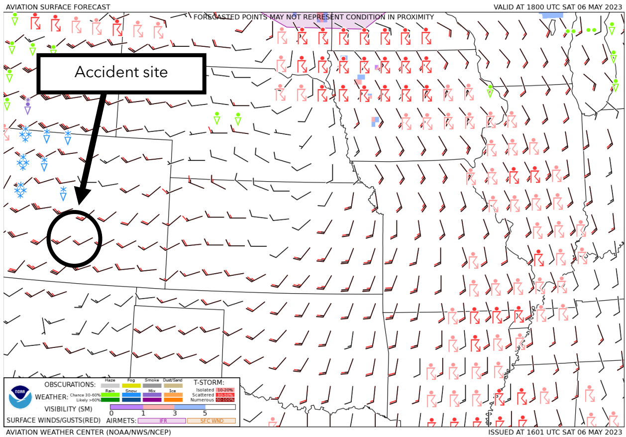
Figure 3. GFA Surface Forecast valid at 1200 MDT with forecast issued at 1001 MDT.
