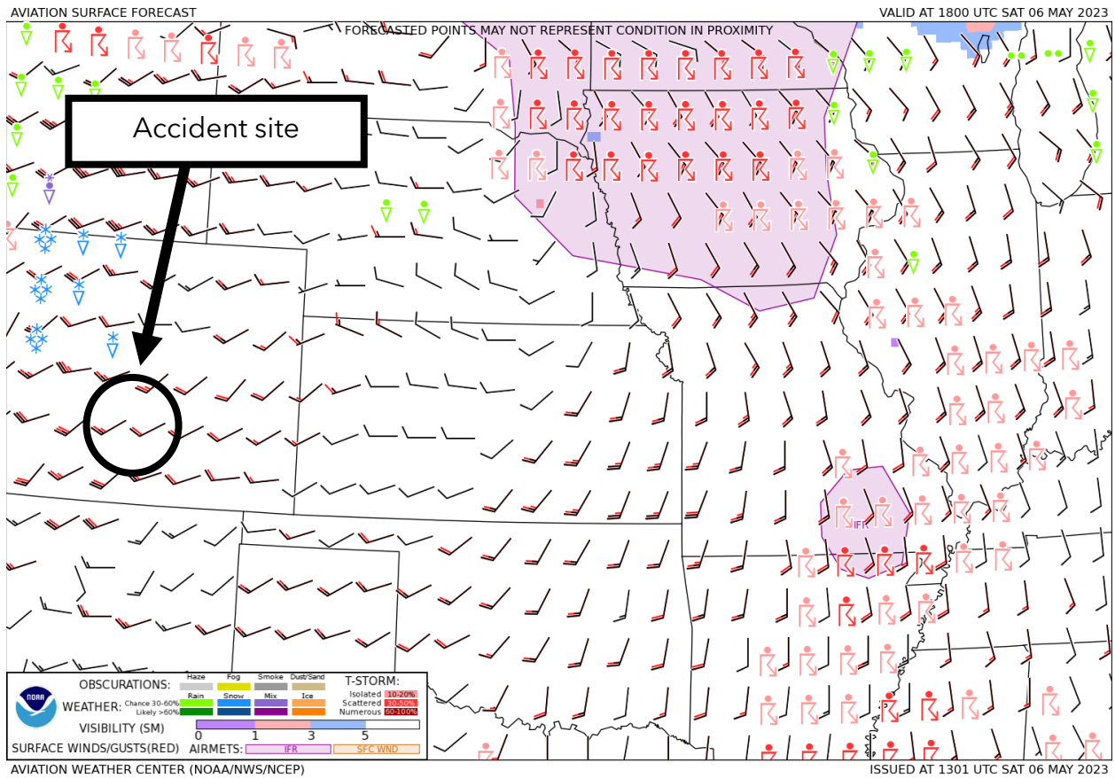
Figure 2. GFA Surface Forecast valid at 1200 MDT with forecast issued at 0701 MDT.
