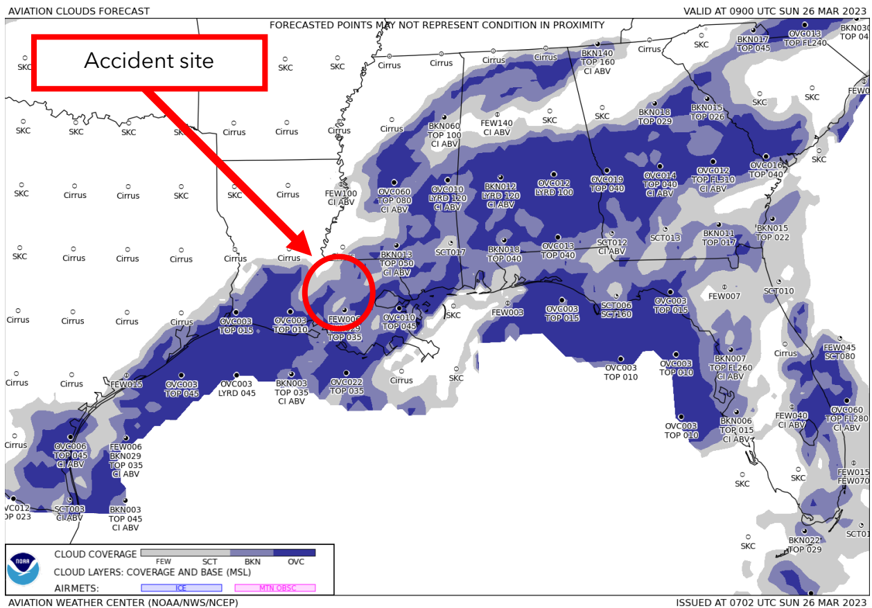
Figure 6. GFA Aviation Clouds Forecast valid at 0400 CDT with forecast issued at 0202 CDT.
