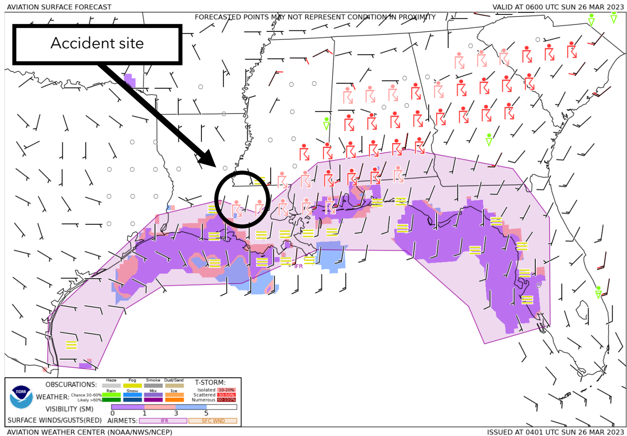
Figure 1. GFA Surface Forecast valid at 0100 CDT with forecast issued at 2301 CDT March 25.
