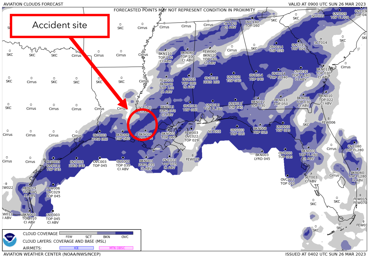
Figure 5. GFA Aviation Clouds Forecast valid at 0400 CDT with forecast issued at 2302 CDT on March 25.
