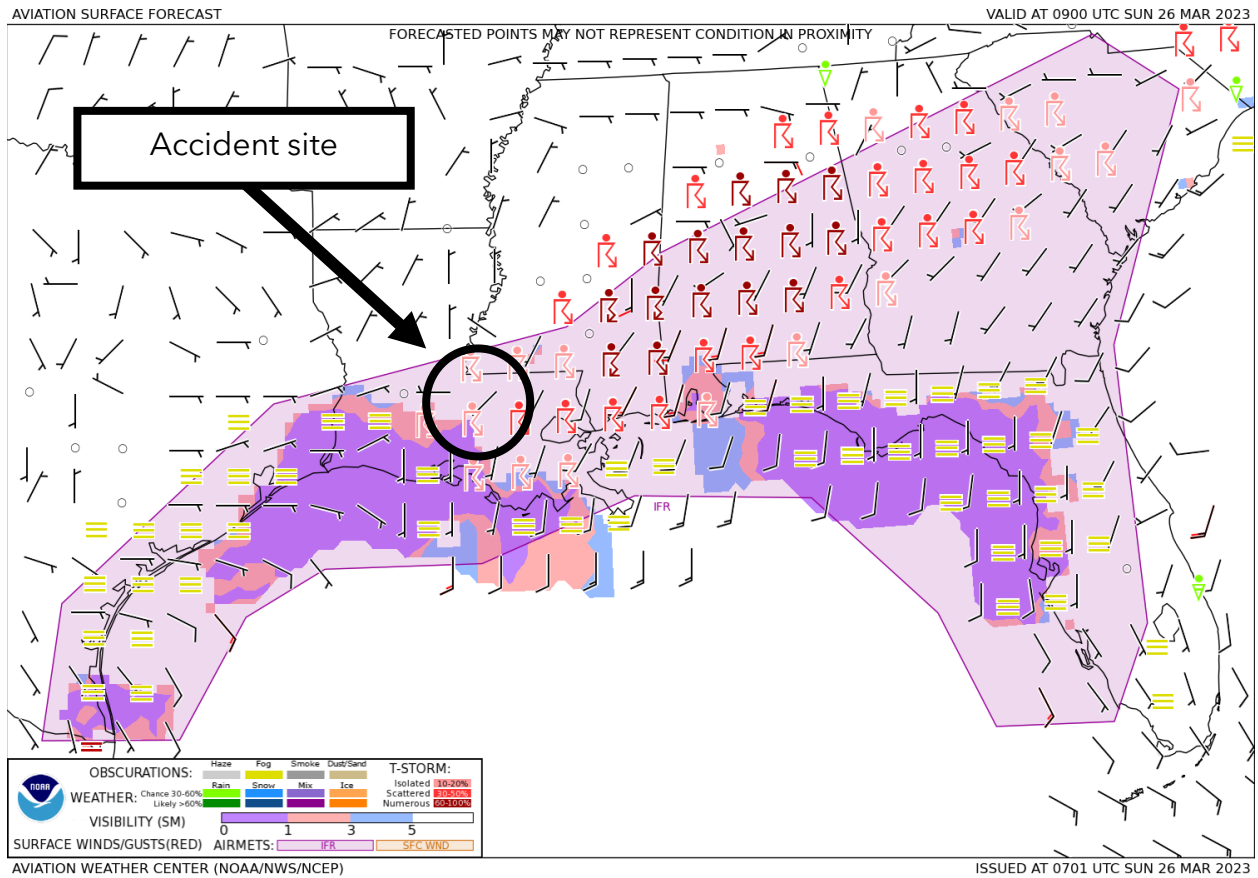
Figure 3. GFA Surface Forecast valid at 0400 CDT with forecast issued at 0201 CDT.
