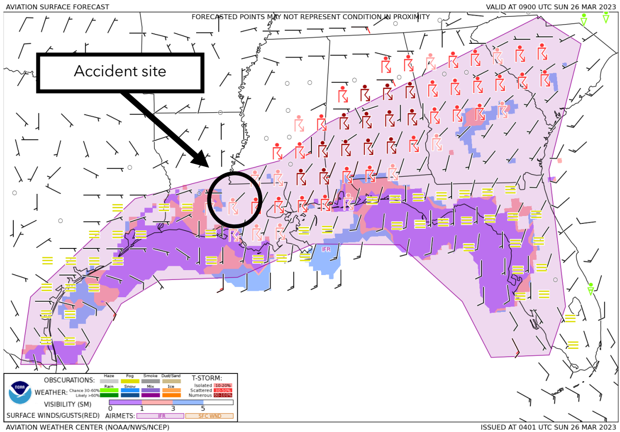
Figure 2. GFA Surface Forecast valid at 0400 CDT with forecast issued at 2301 CDT on March 25.
