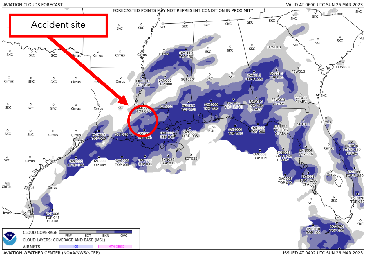
Figure 4. GFA Aviation Clouds Forecast valid at 0100 CDT with forecast issued at 2302 CDT on March 25.
