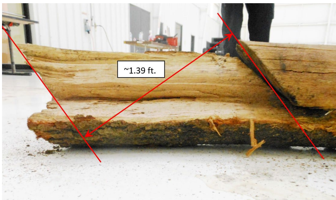
Photograph 3 - Tree Limb Section Showing Propeller Blade Cut
