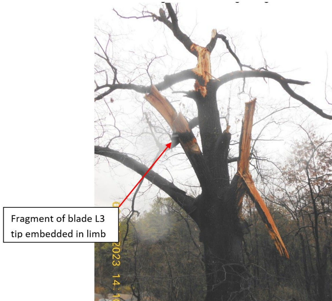
Photograph 2 - Fragment of Propeller Blade Embedded in a Tree Limb
