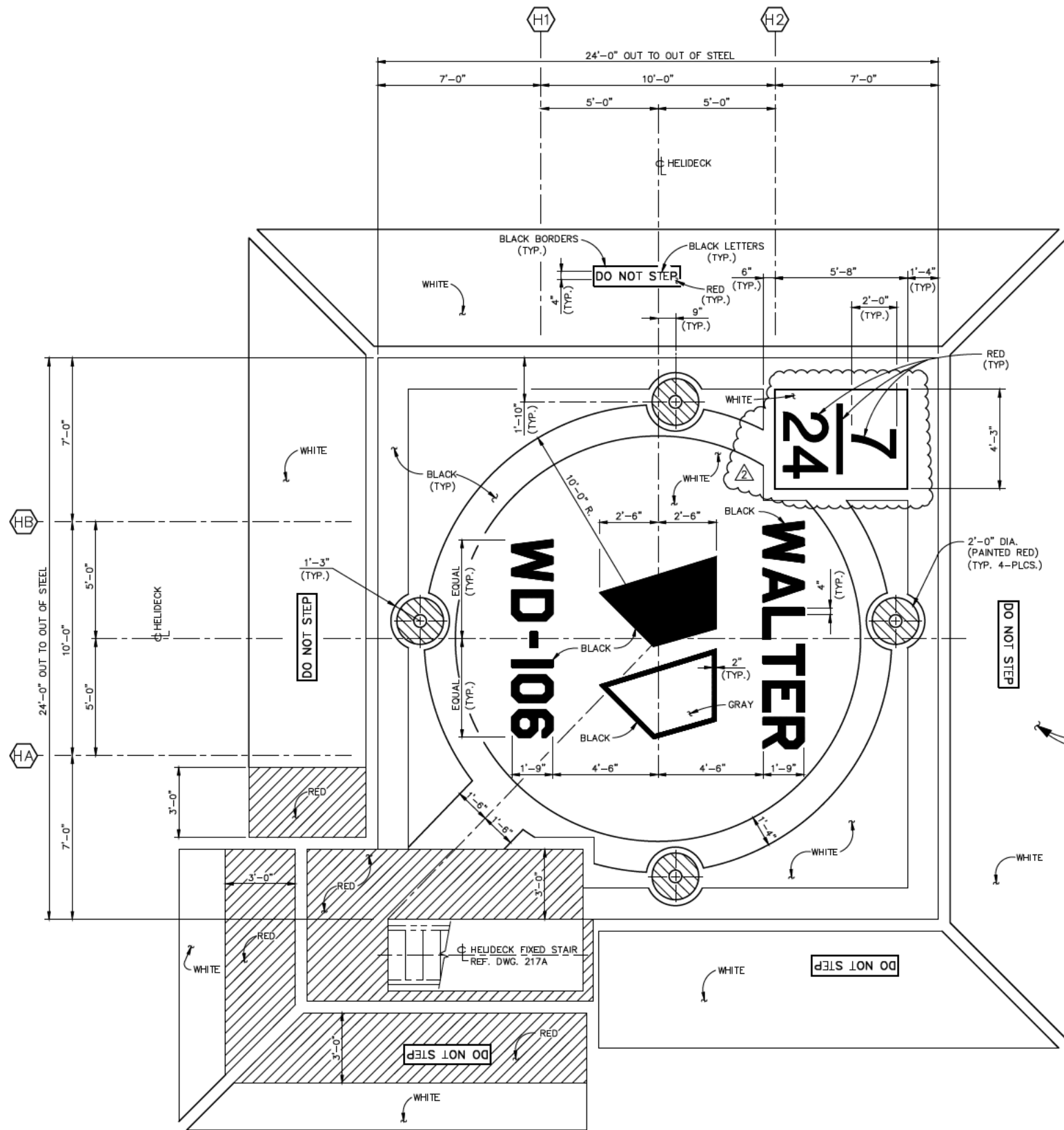
HELIDECK MARKINGS PLAN SCALE 3/8" = 1'-0"
