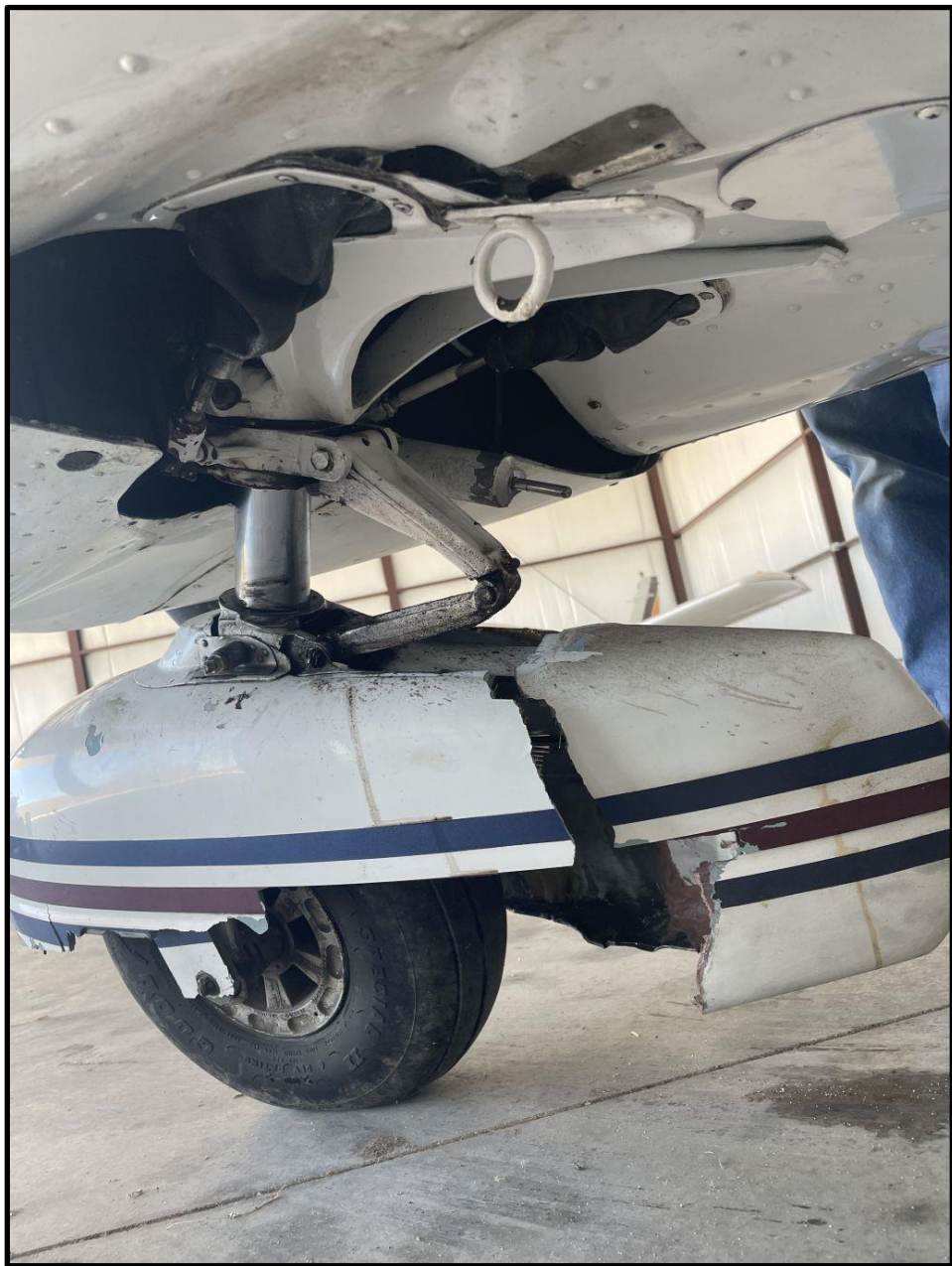
Photo 4 – Lower Fwd Fuselage / Nose Landing Gear (FAA Photo)
