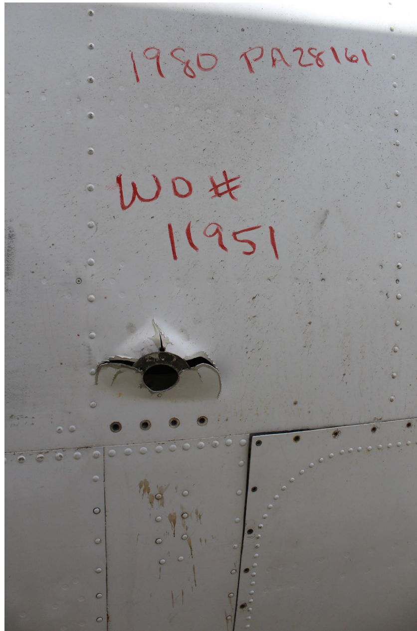
Photo 4 – View of the top of the left wing (courtesy of The New Firewall Forward).
