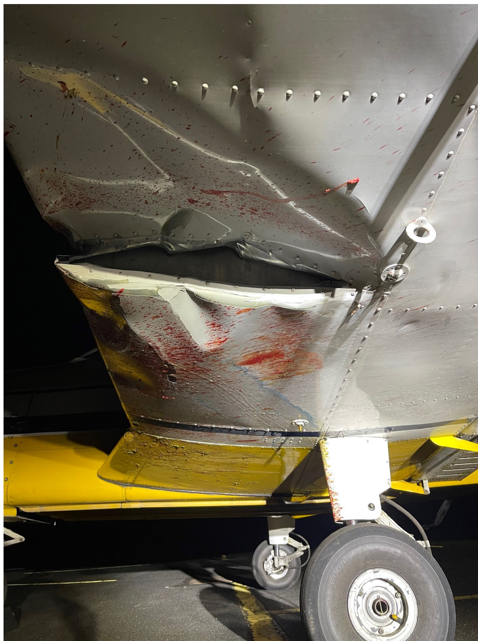
Accident Airplane / Bottom Left Wing / Landing Gear – (Photo provided by the pilot)
