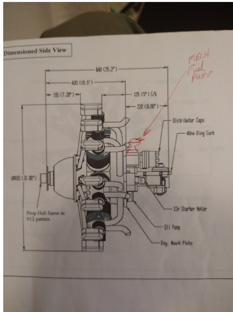
Photo 3 – Engine Drawing (Provided by Owner)
