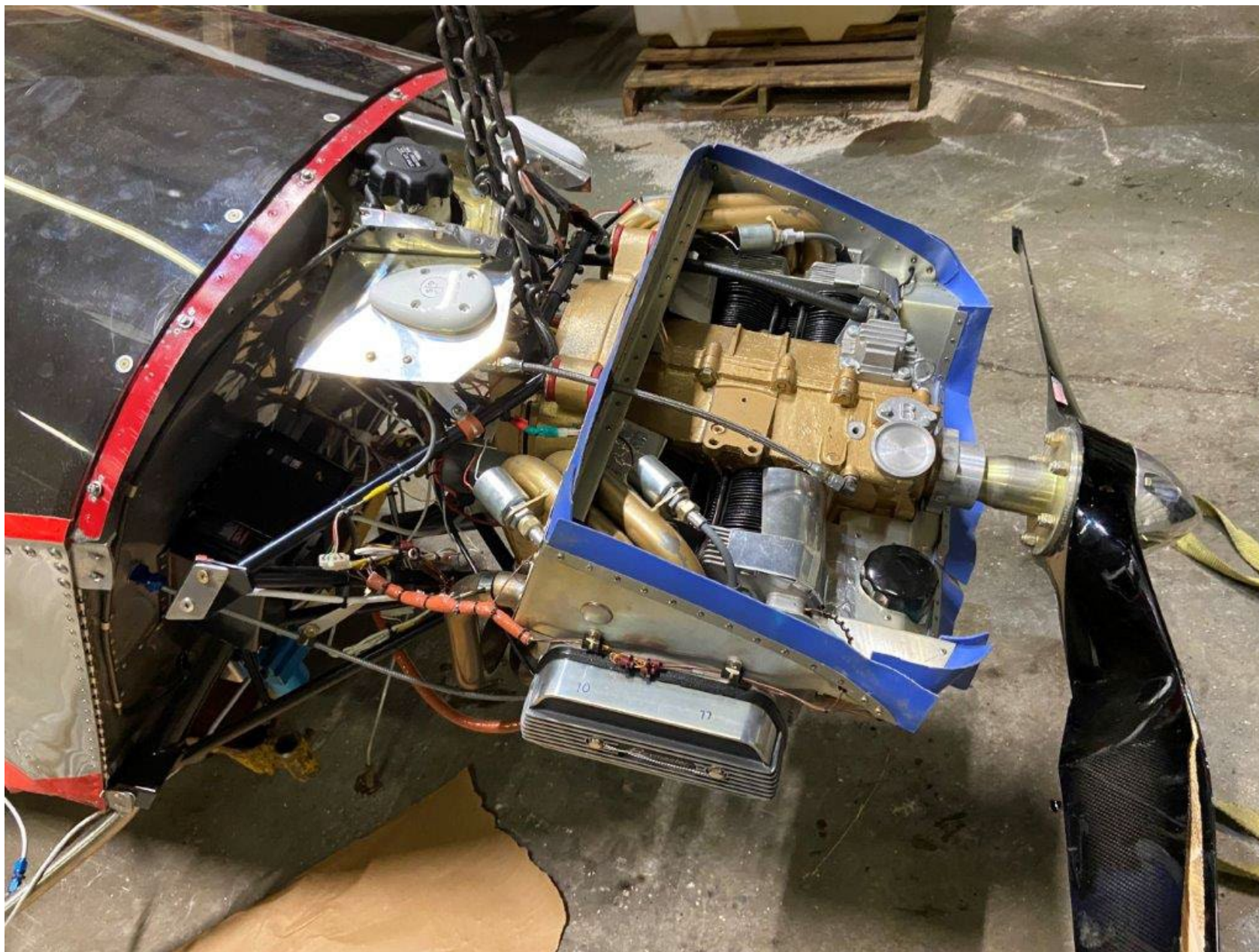
Photo 9 – View of the right side of the engine at the salvage facility (courtesy of the Federal Aviation Administration).
