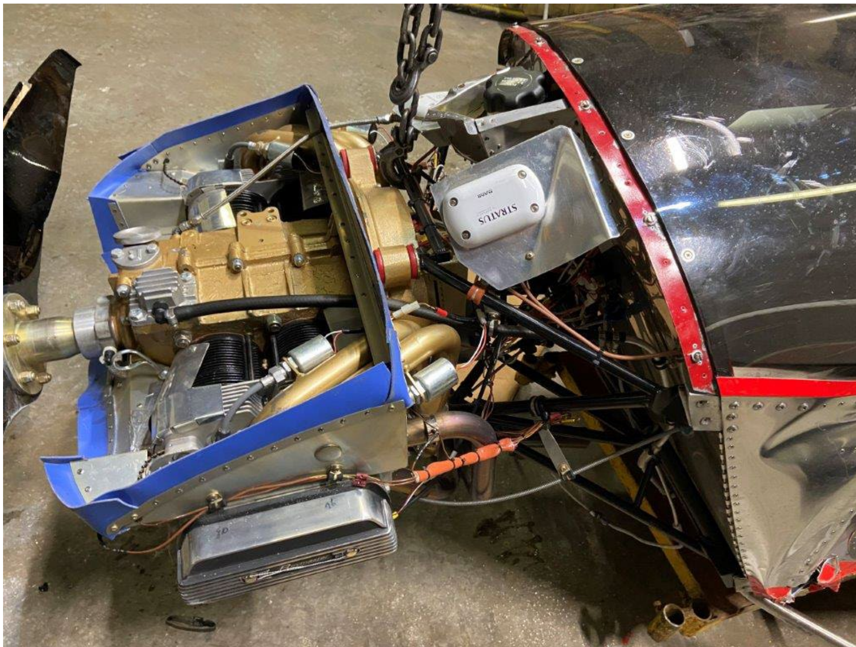
Photo 10 – View of the left side of the engine at the salvage facility (courtesy of the Federal Aviation Administration).
