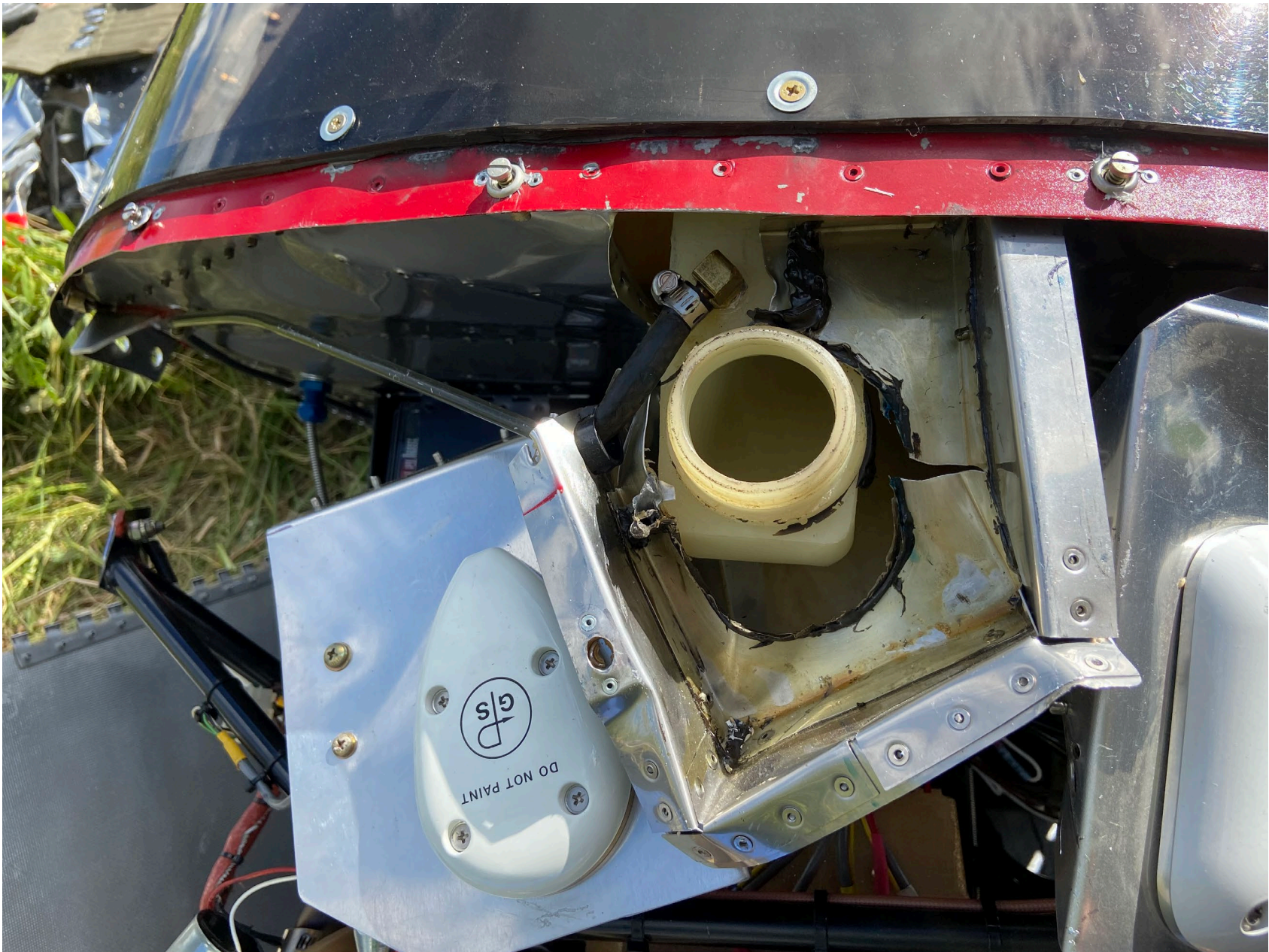
Photo 4 – View of the fuel tank at the accident site, with the fuel tank cap removed (courtesy of the Federal Aviation Administration).
