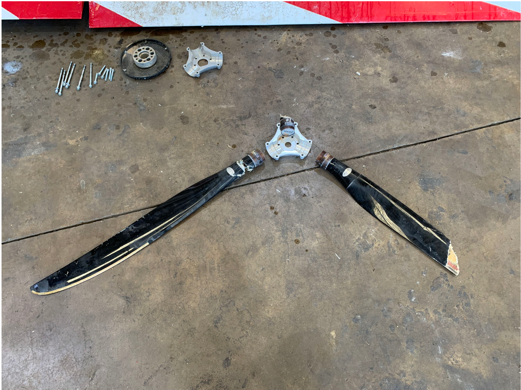
Photo 17 – View of the propeller.
