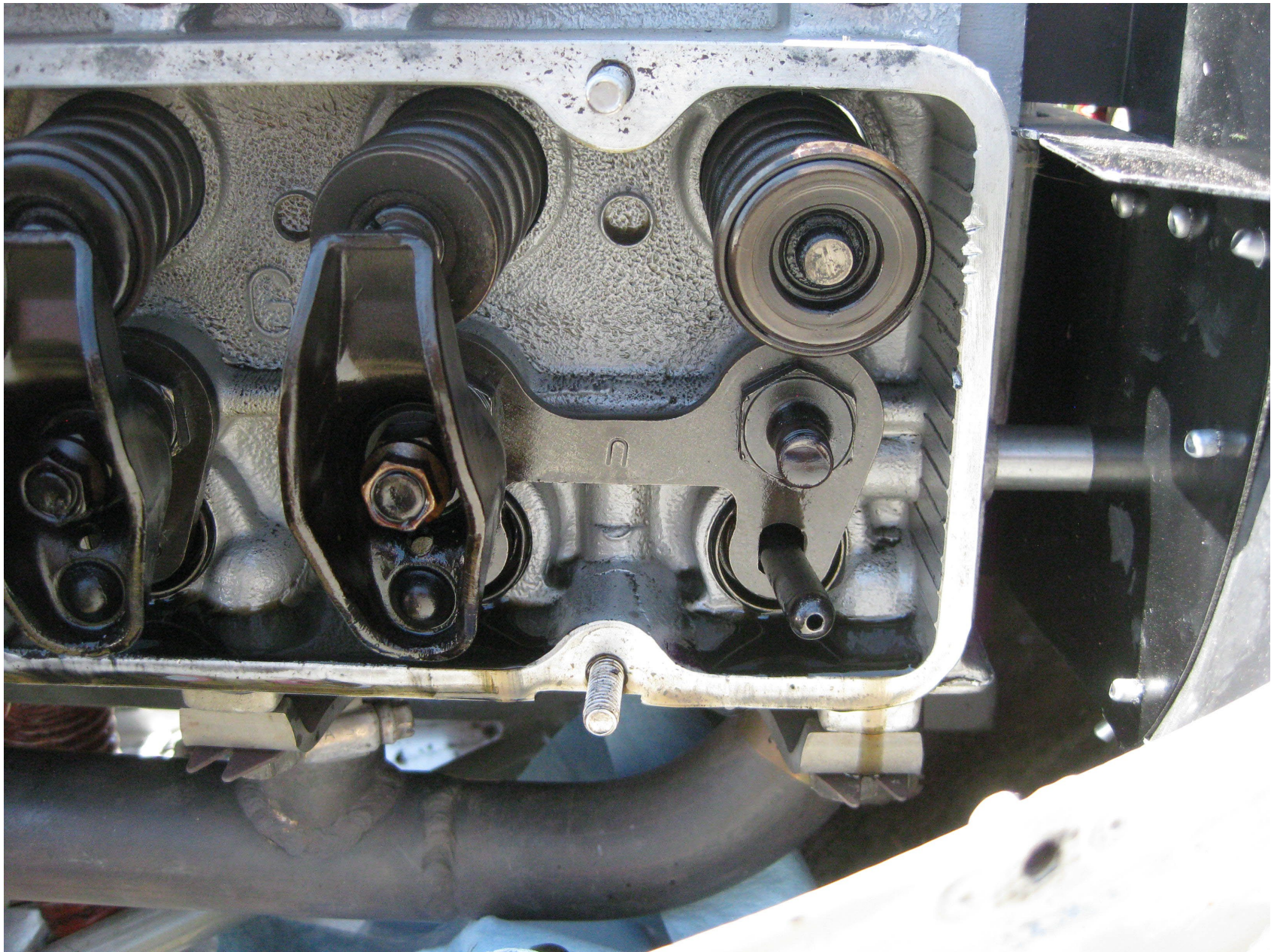
Photo 1 – No. 5 Cylinder and Rocker Arm (photograph provided by airplane owner)
