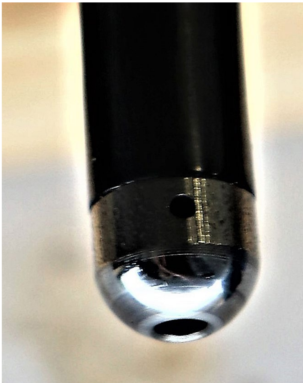
Photo 3 - End of Push Rod (photograph provided by airplane owner)
