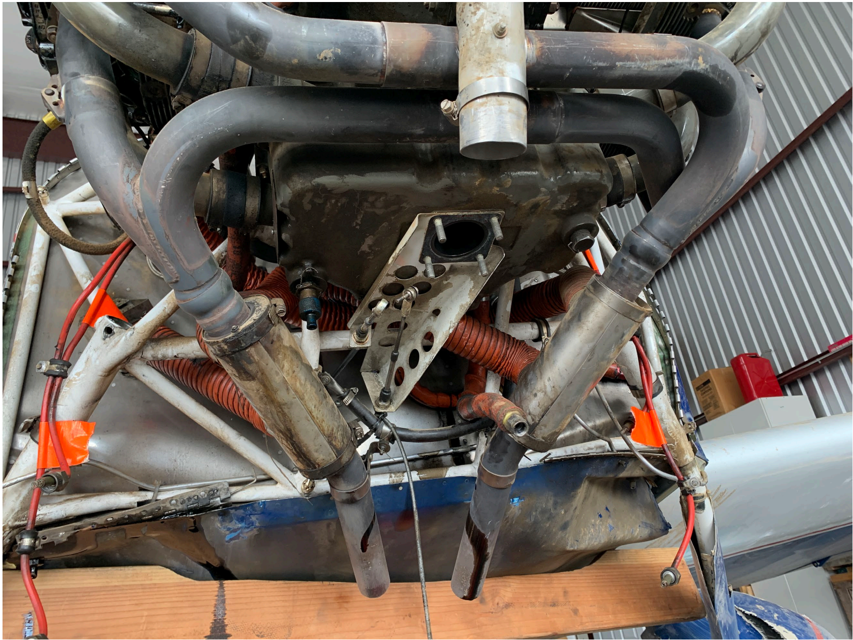
Photo 5 – View of the substantial damage sustained to the area behind the firewall and to the lower fuselage.
