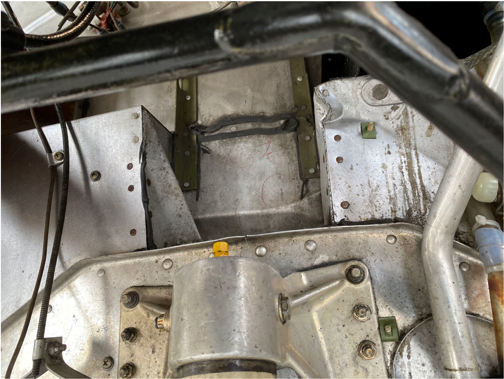
Photo 2 – View of the damage sustained to the firewall (courtesy of the Federal Aviation Administration).
