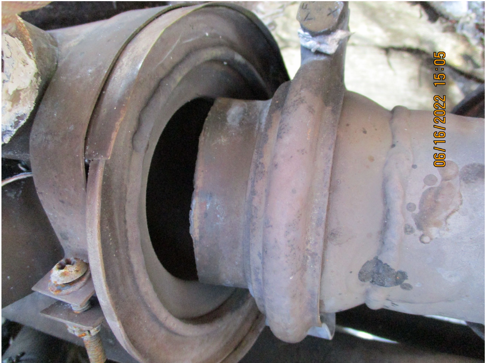
Photo 4 – Closer View of Exhaust Components at Initial Exam, Courtesy of FAA
