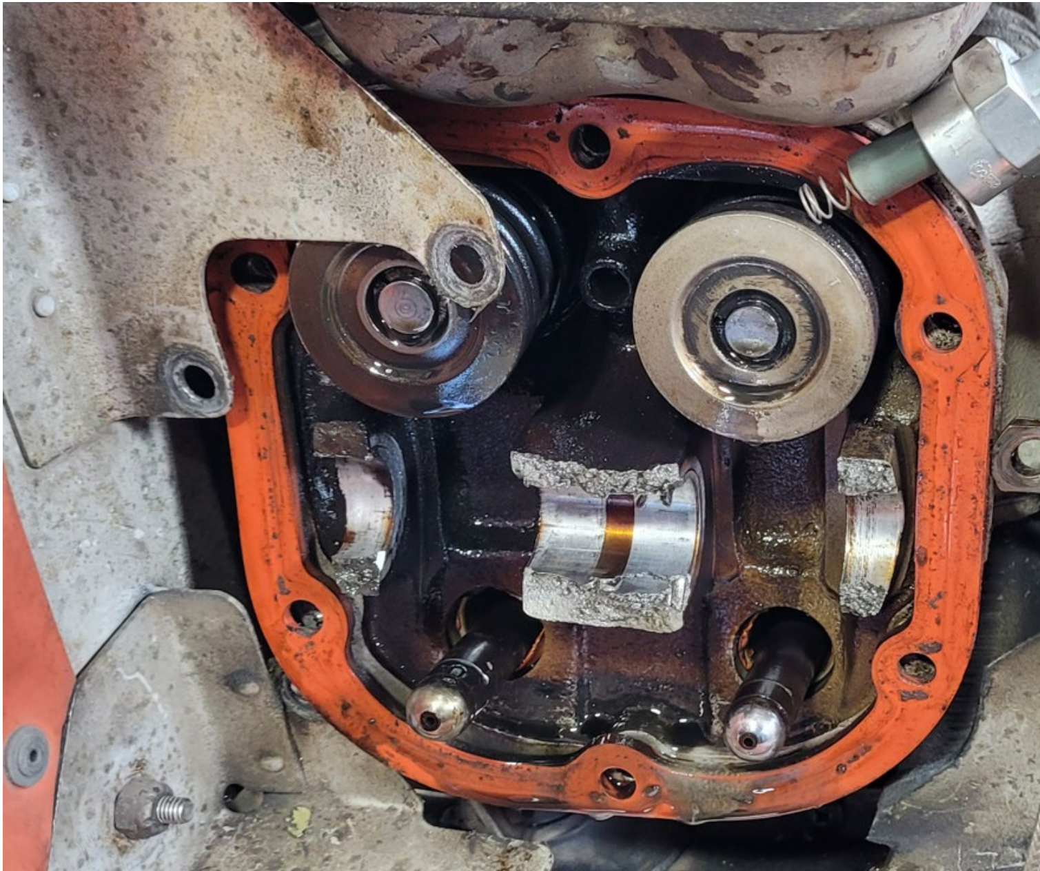
Photo 2 – Fractured No. 1 Cylinder Shaft Rocker Bosses, Courtesy of FAA
