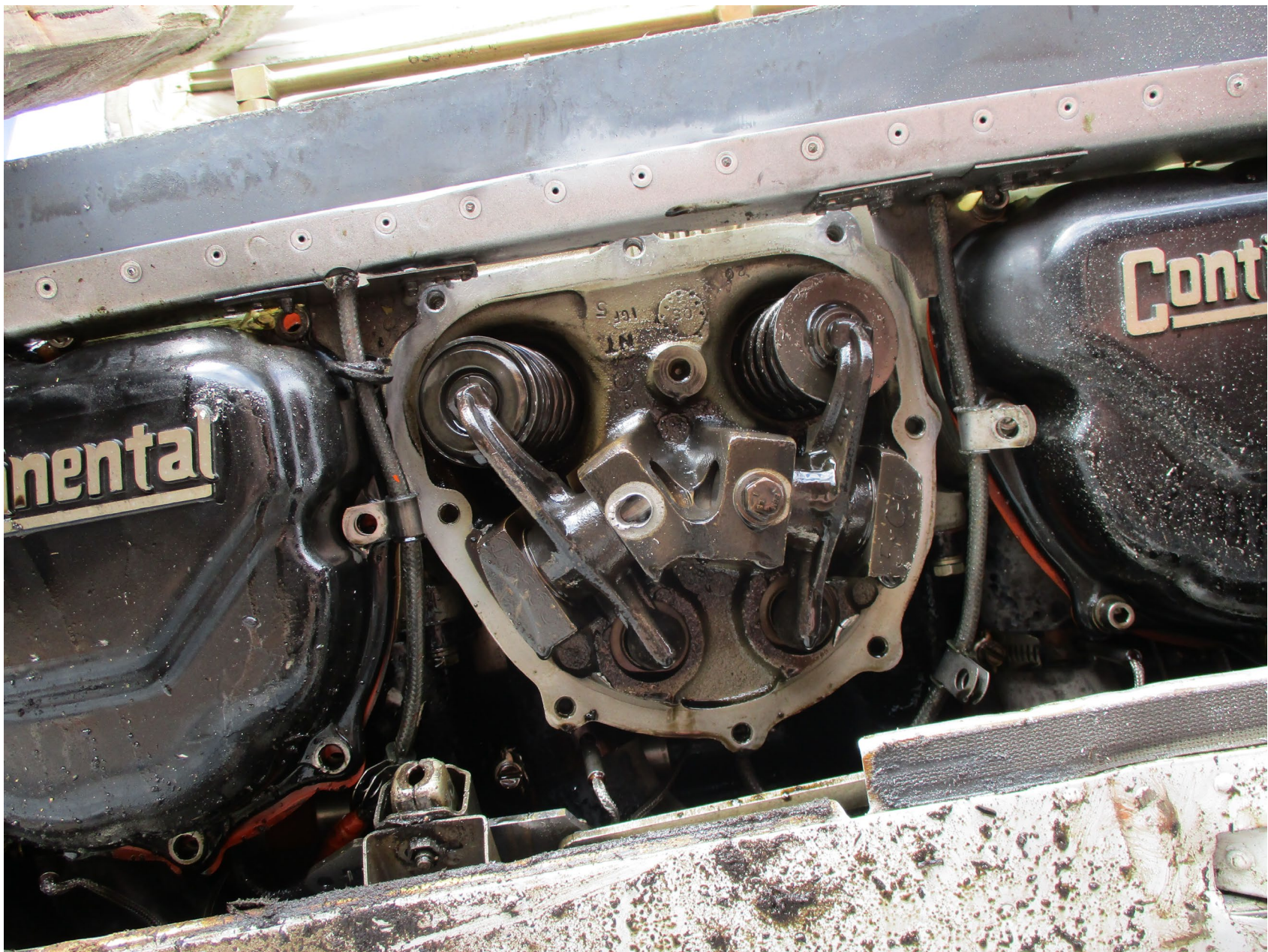
Photo 6 – View of No. 4 cylinder head (FAA Photo)
