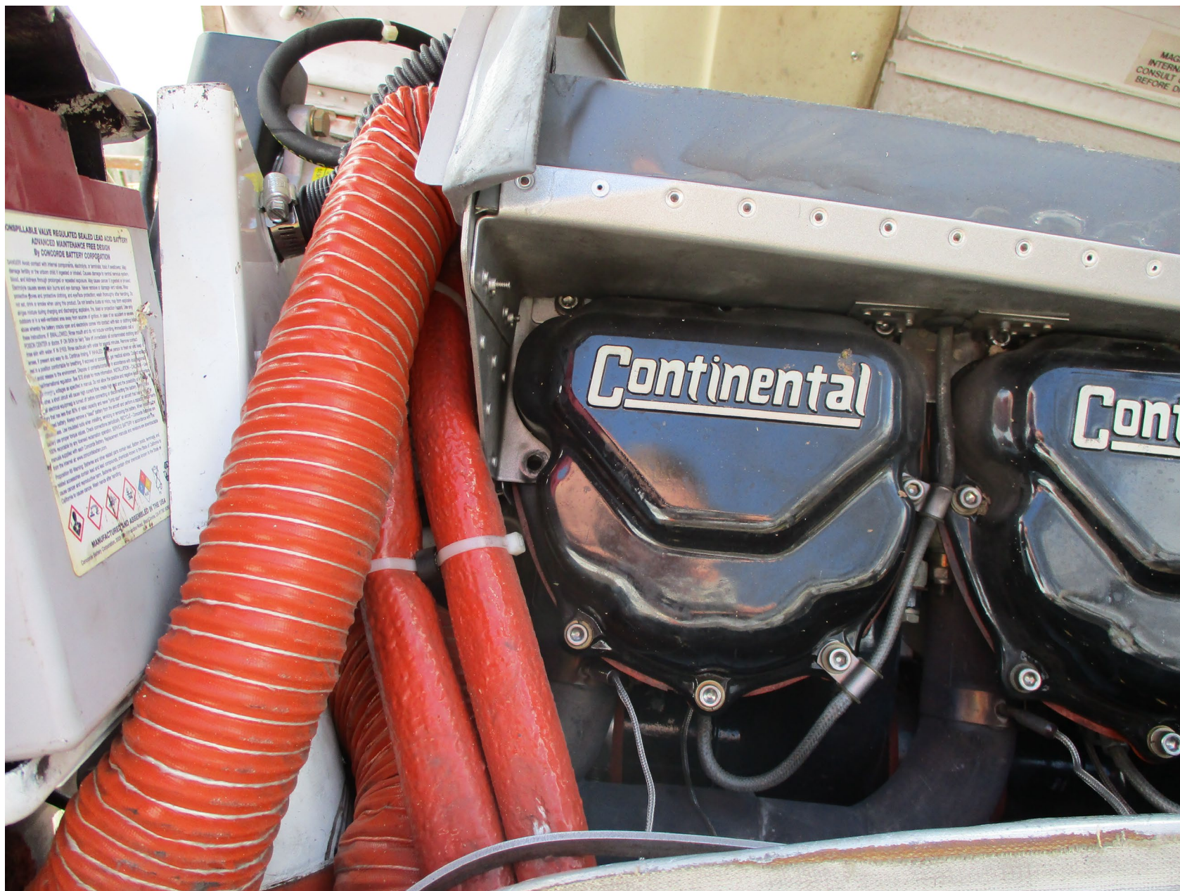
Photo 5 – View of No. 5 rocker cover showing missing bolt (FAA Photo)
