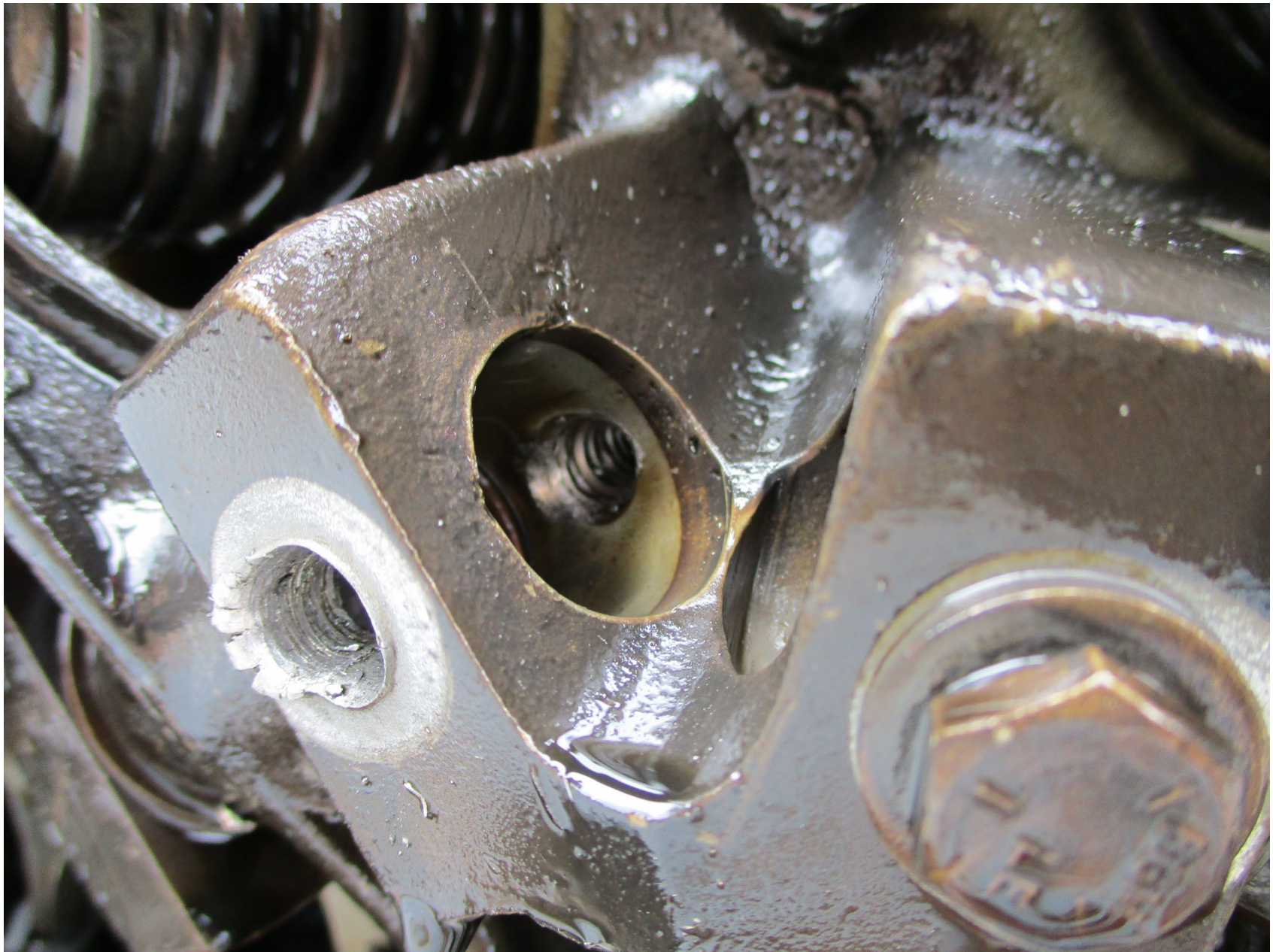
Photo 8 – No. 4 rocker arm shaft boss (FAA Photo)
