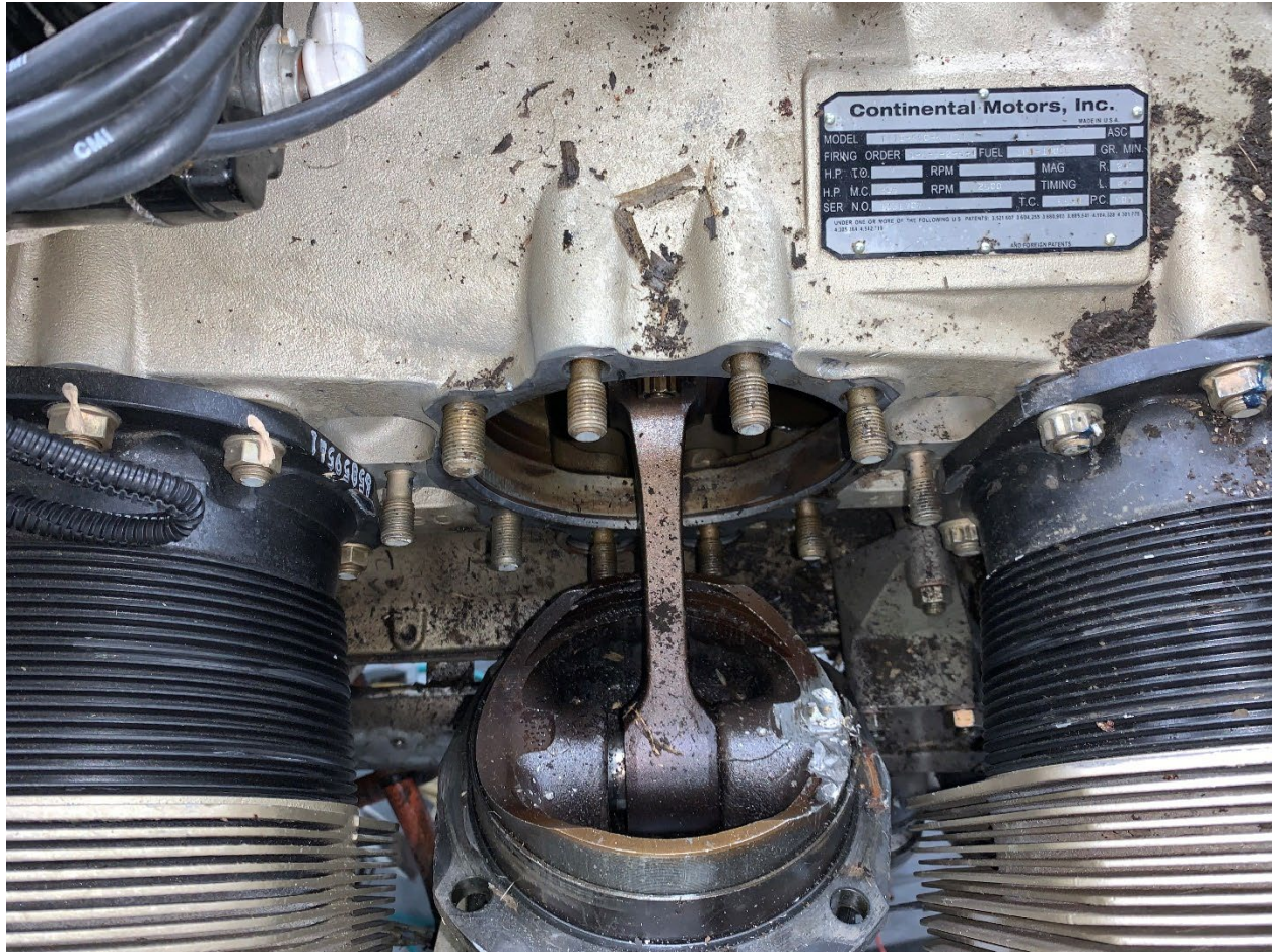
Photo 3: Number 3 Cylinder Piston (Source – NTSB IIC)
