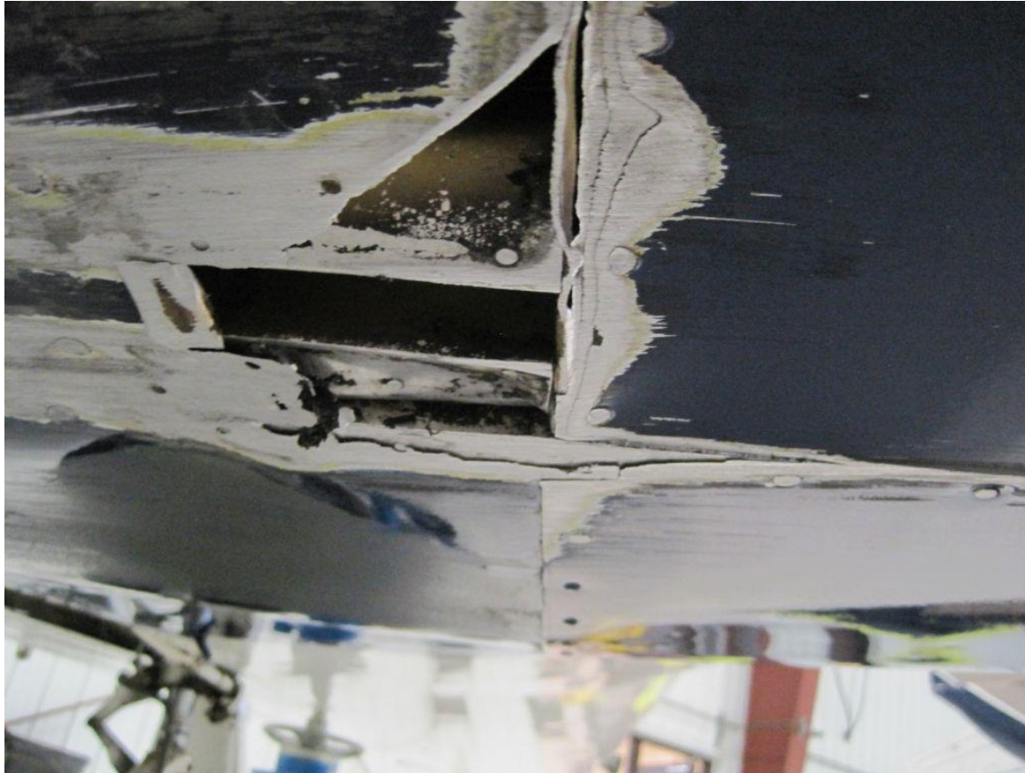
Photograph 5 - Lower Fuselage (FAA Photo)
