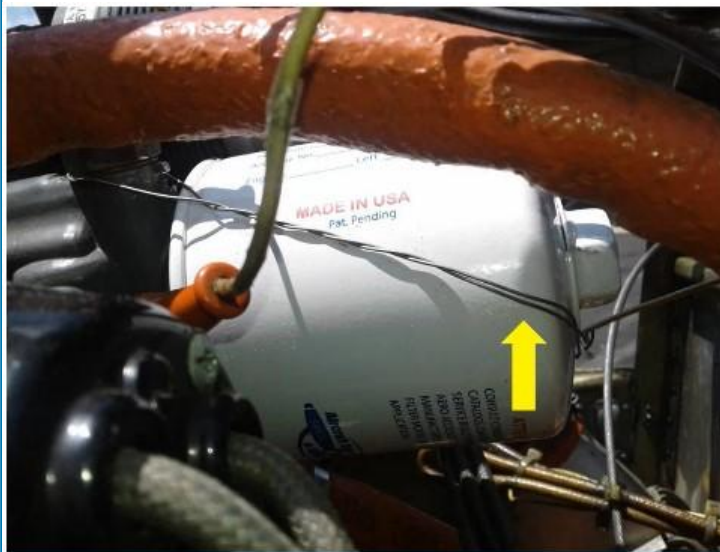
This oil filter was not properly safety wired. The wire is routed in the right direction, but there are too few twists per inch. The arrow points to the section with no twist.
