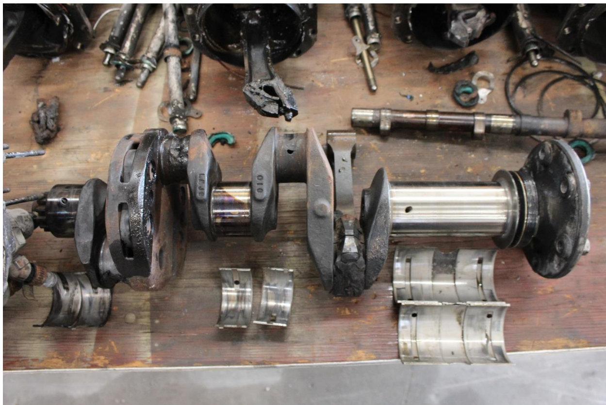
Photo 5: Crankshaft (NTSB Photo)
