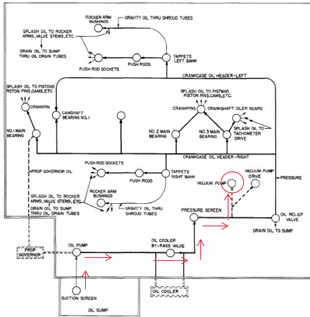
Figure 2-3. Lubrication Diagram - 4 Cylinder Engines
