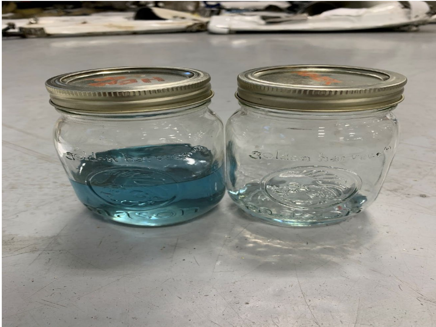
Photograph 5 - Header Tank Contents (NTSB)
