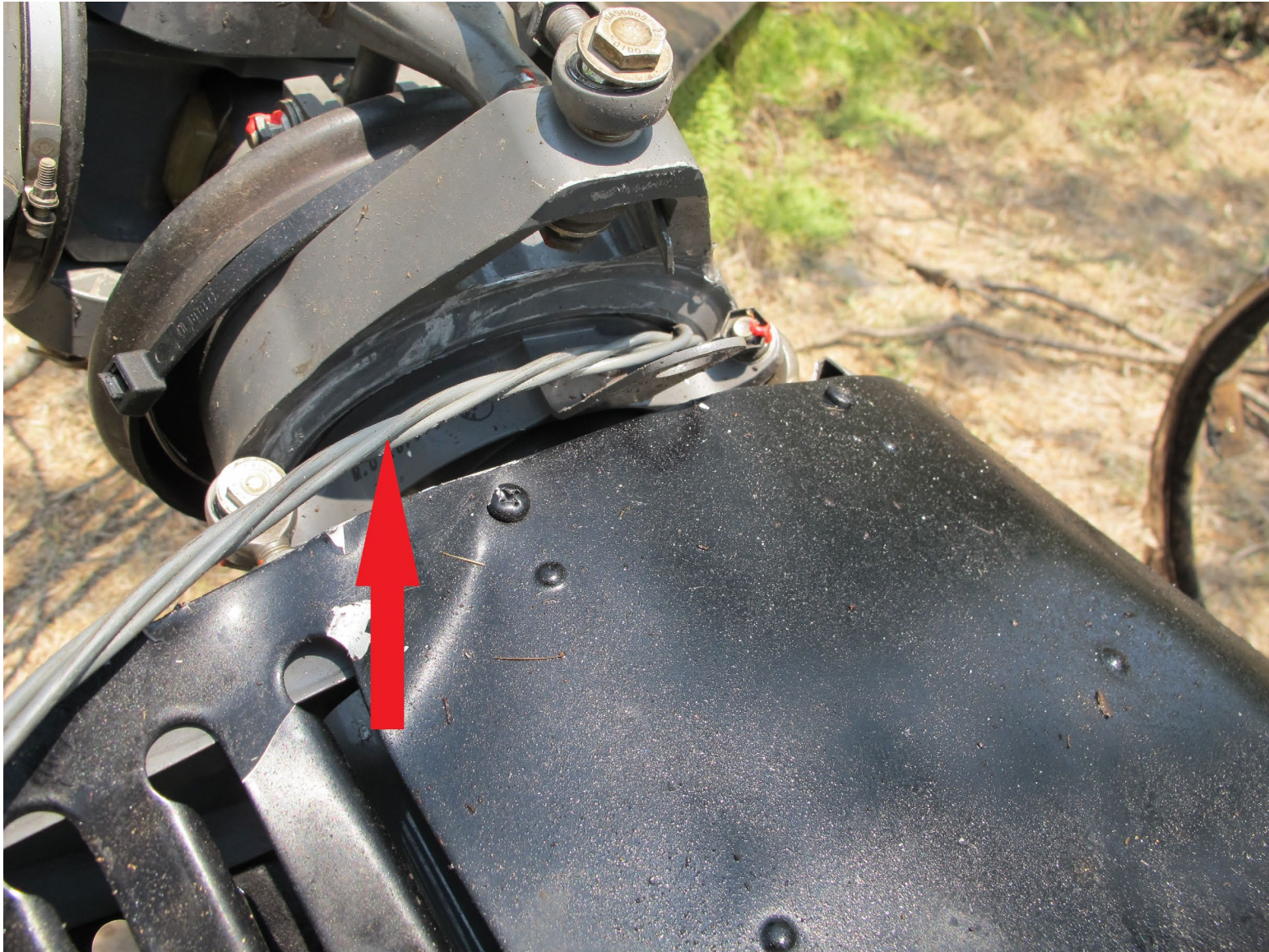
Photograph 6 - Wire Wrapped Around Leading Edge of Swashplate (Courtesy of NTSB)
