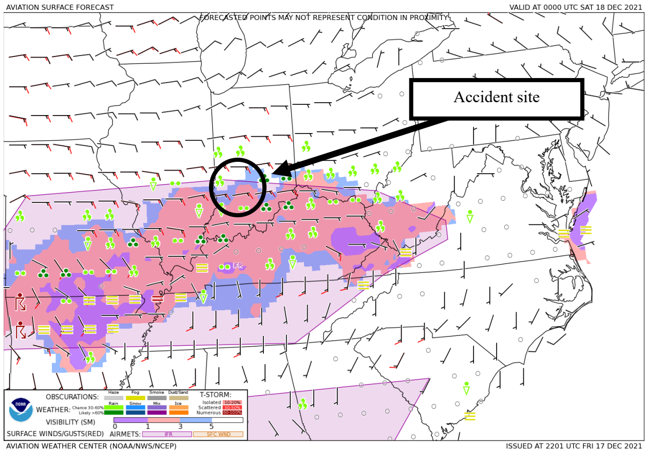
Figure 2 – GFA Surface Forecast valid at 1900 EST with forecast issued at 1701 EST.
