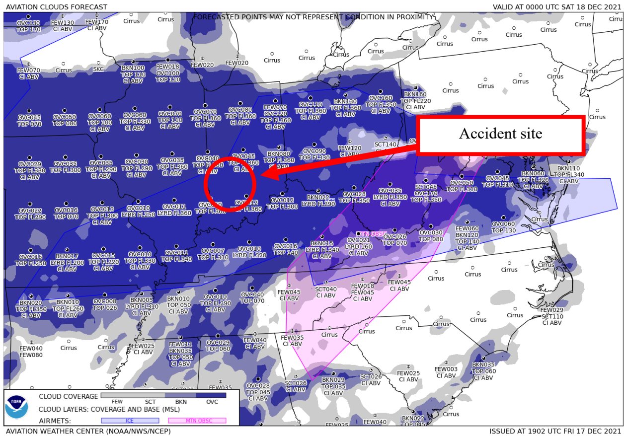
Figure 3 – GFA Aviation Clouds Forecast valid at 1900 EST with forecast issued at 1402 EST.
