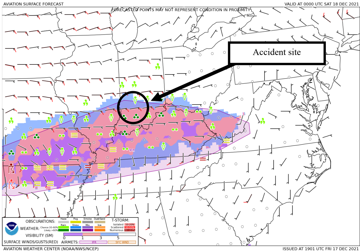
Figure 1 – GFA Surface Forecast valid at 1900 EST with forecast issued at 1401 EST.
