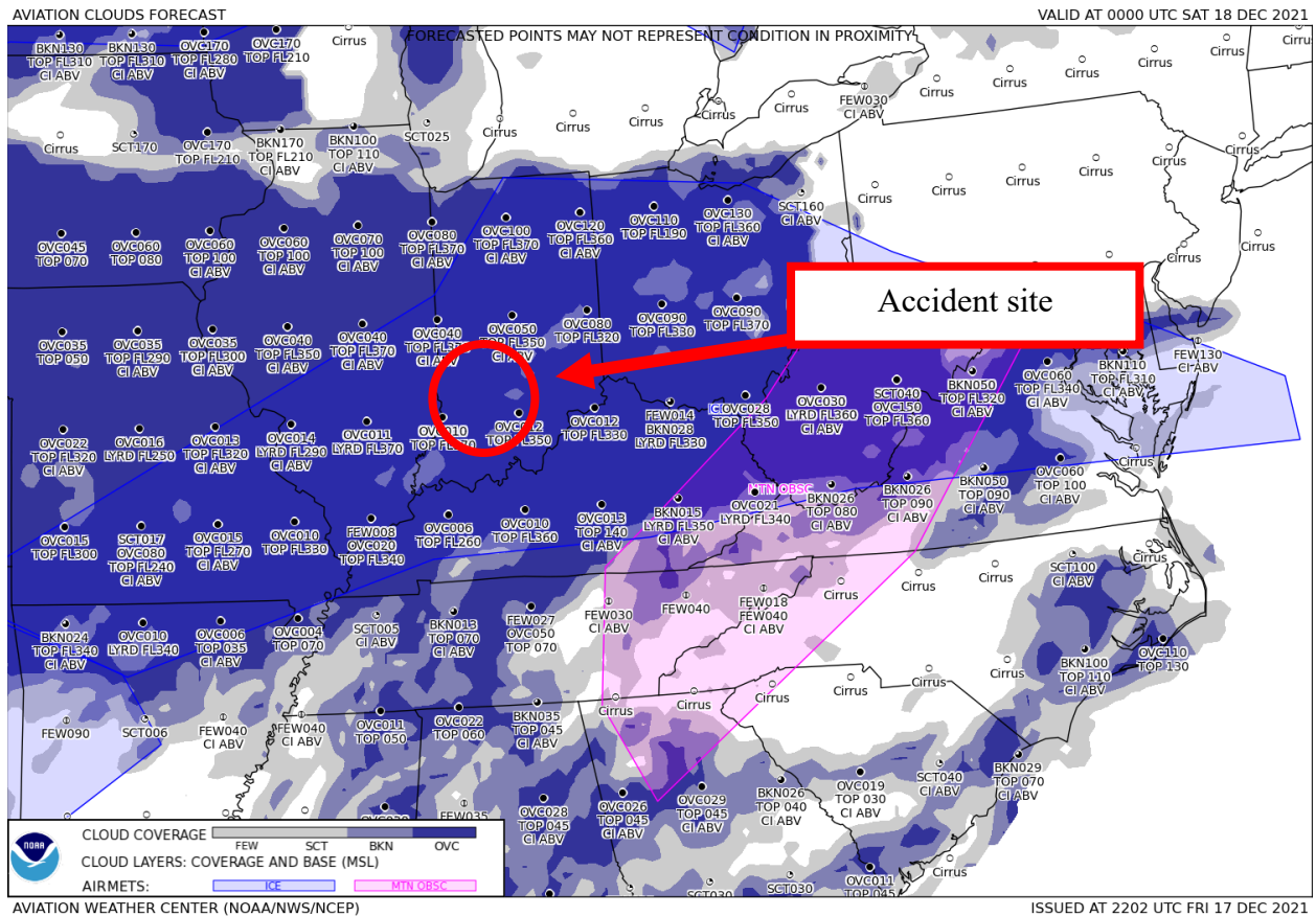
Figure 4 – GFA Aviation Clouds Forecast valid at 1900 EST with forecast issued at 1702 EST.
