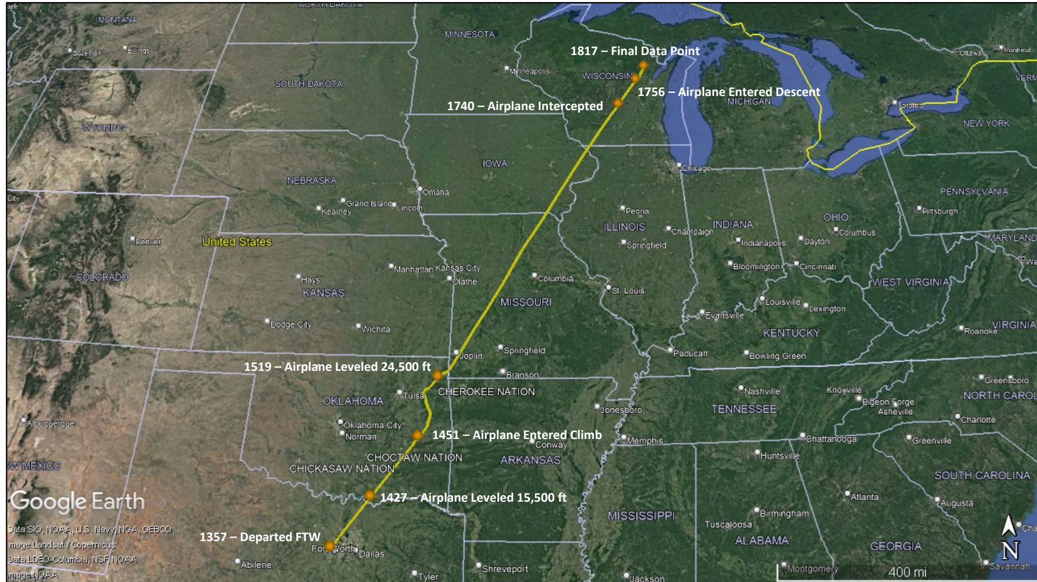
Figure 1 – Accident Flight Overview
