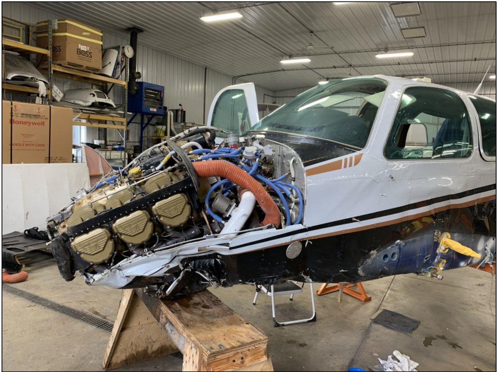
Photo 4 – Forward Fuselage / Engine
