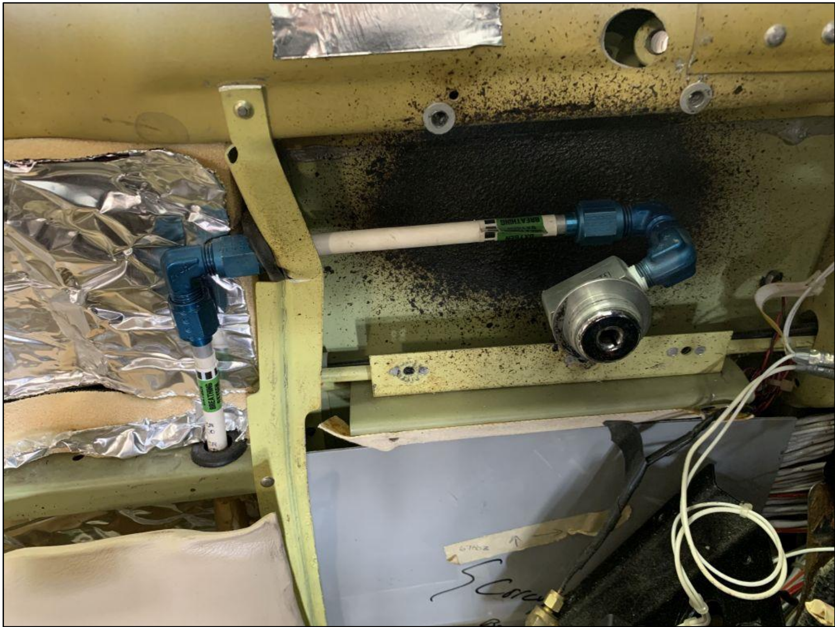
Photo 5 – Pilot-Side Oxygen Line
