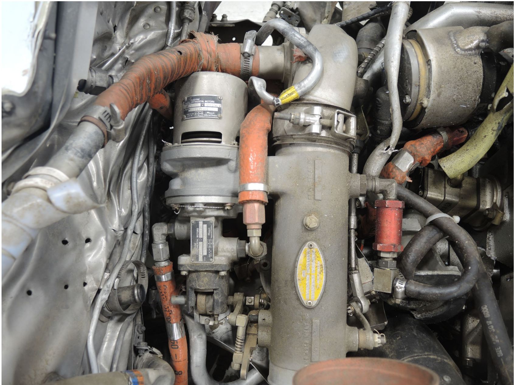
Photo 15 – Right Engine Throttle and Control Assembly
