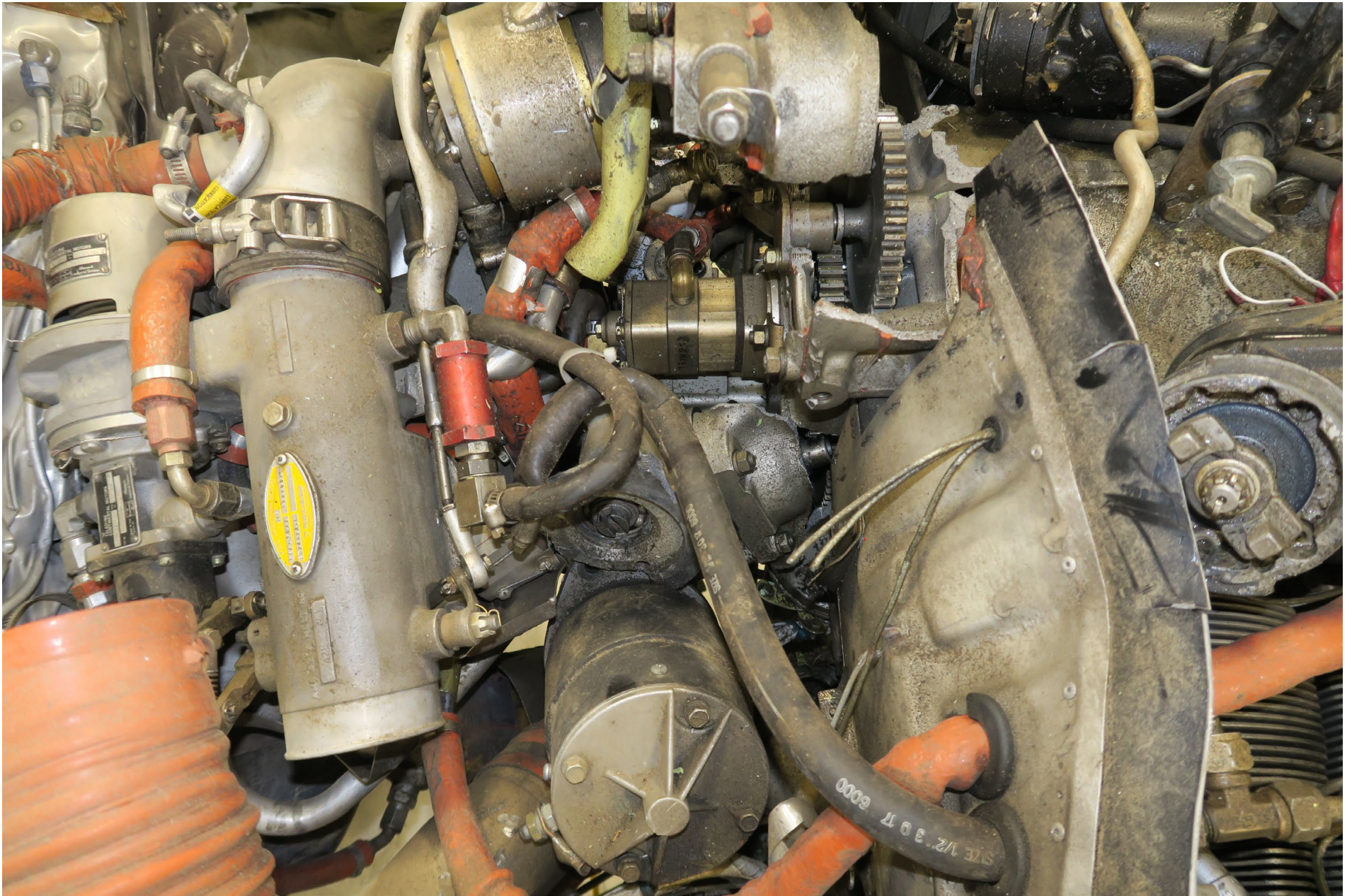
Photo 13 – Right Engine Accessories
