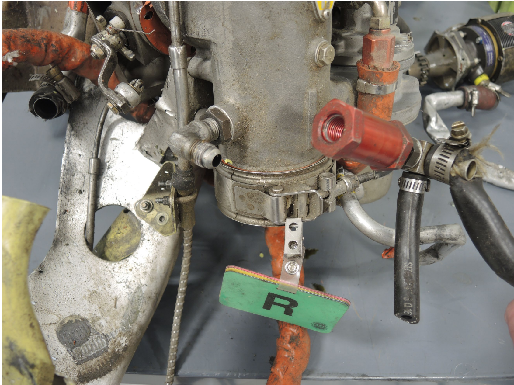
Photo 16 – Right Engine Turbo Controller Check Valve
