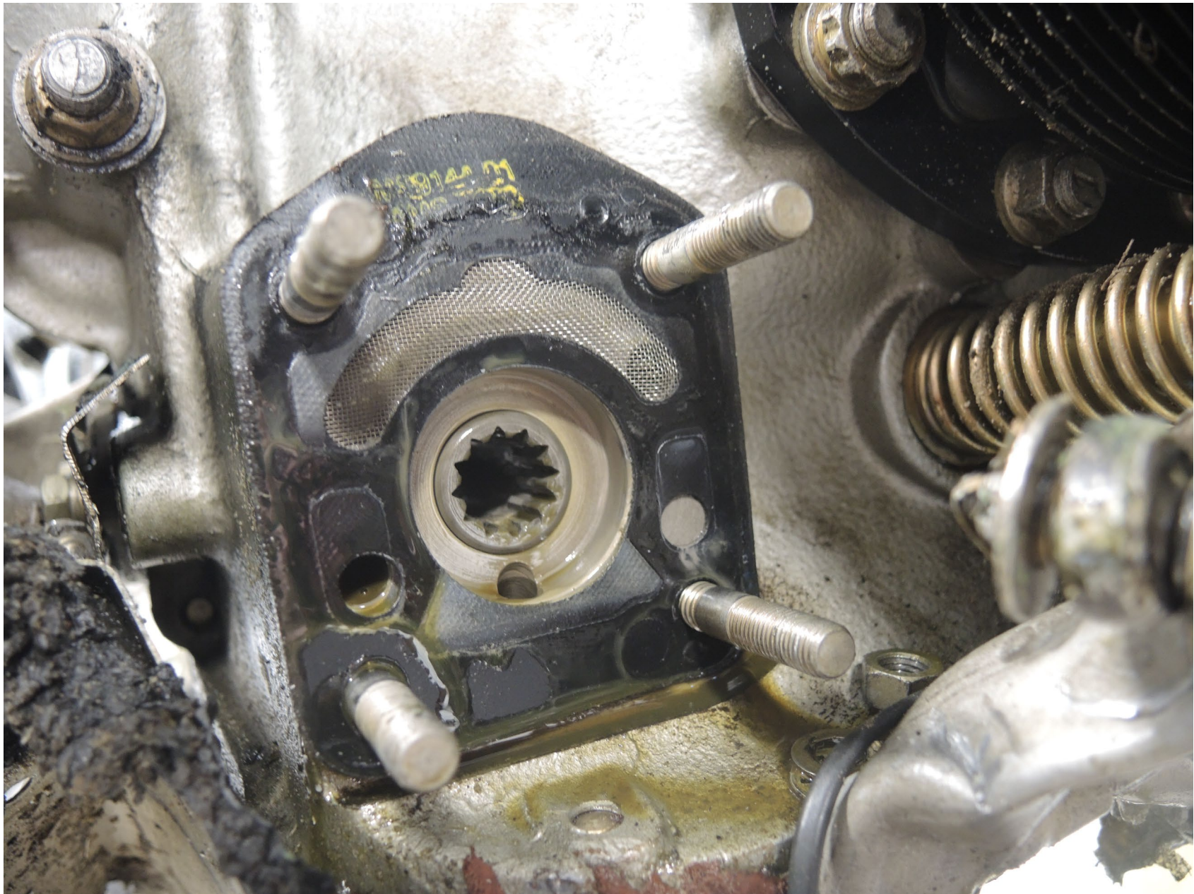
Photo 18 – Propeller Governor Mounting Pad
