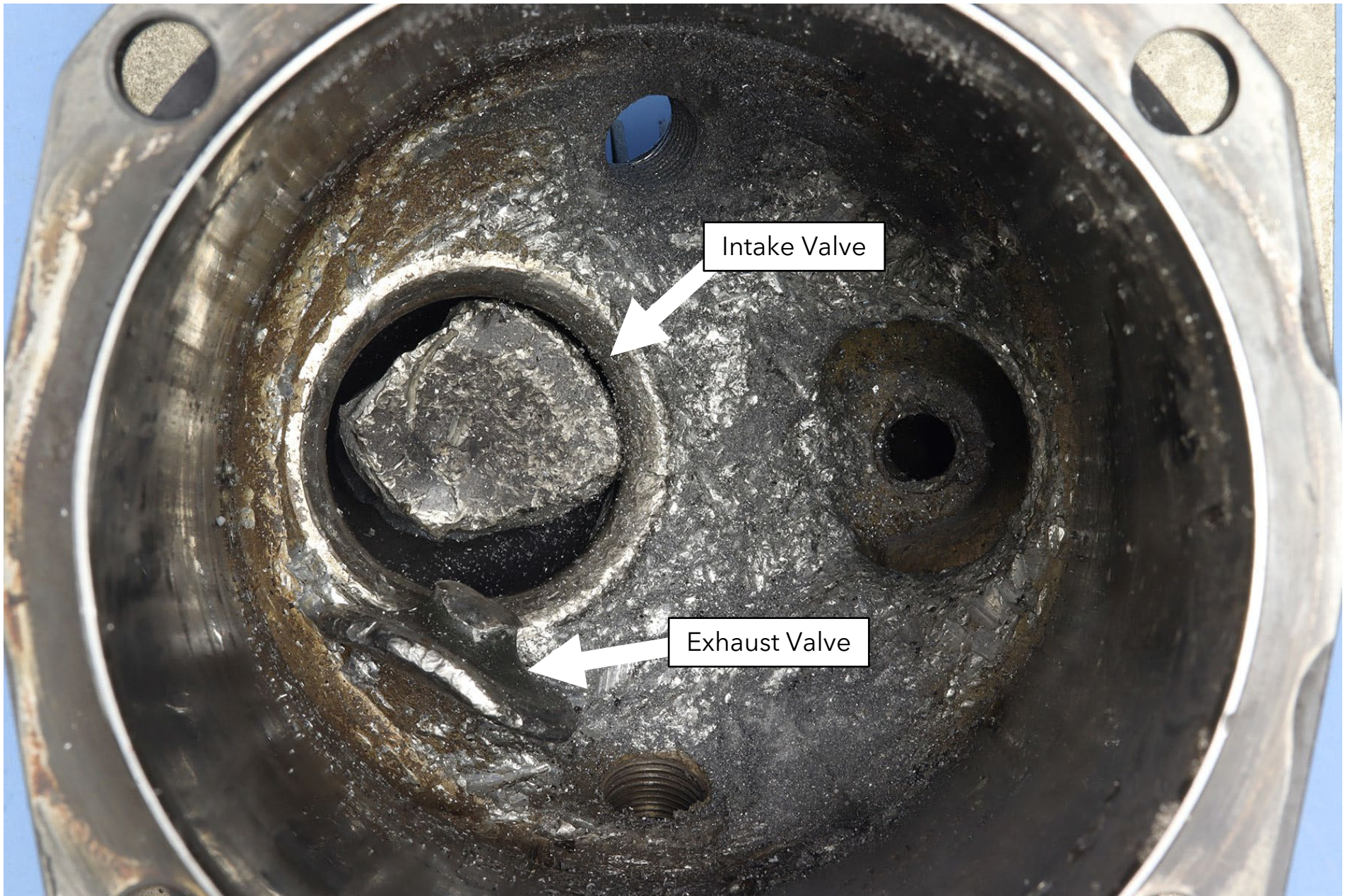
Photo 4 - Inside No. 2 Cylinder (NTSB Photo)
