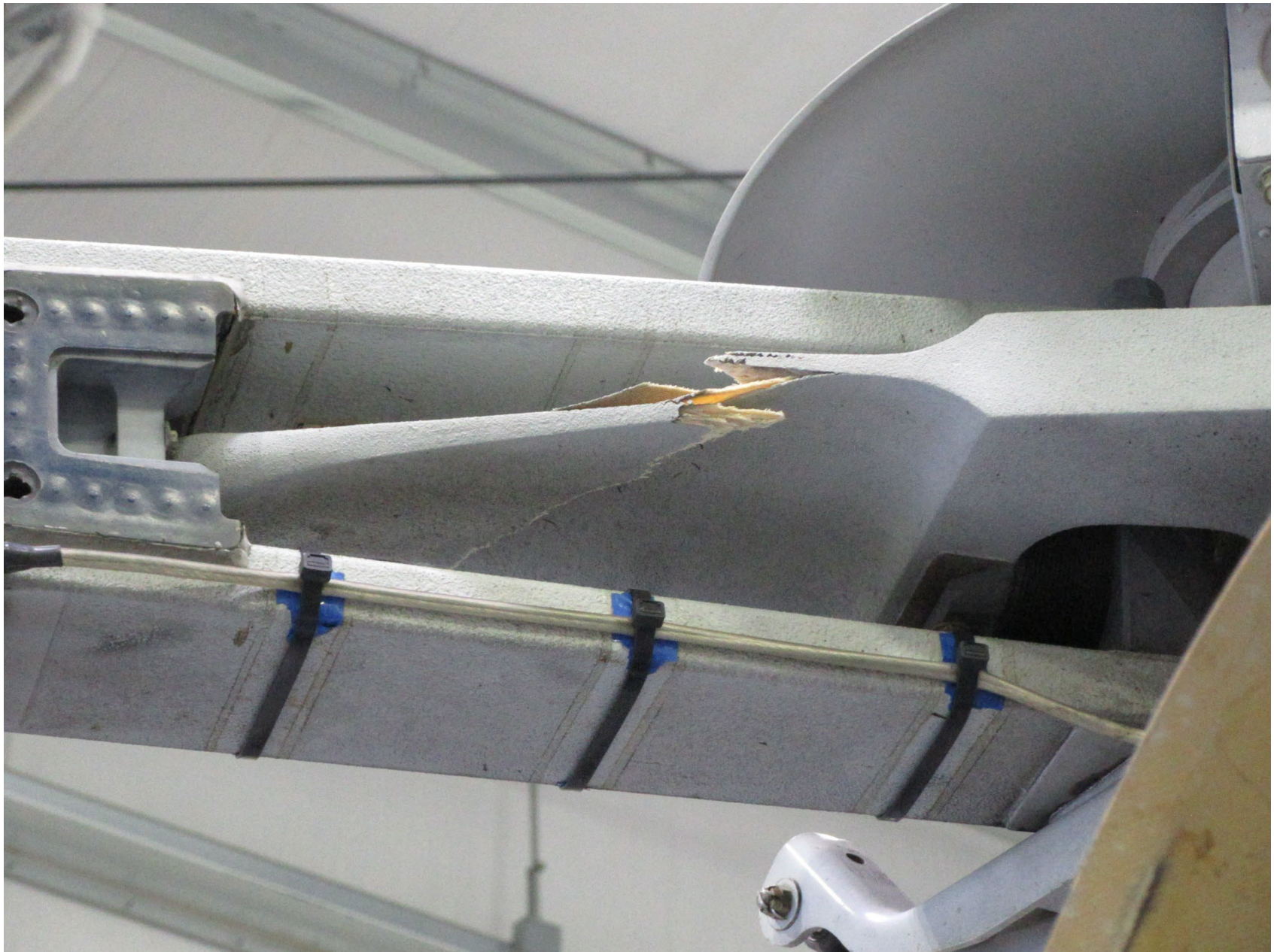
Photo 2 - Blue Main Rotor Blade Starflex Fracture
