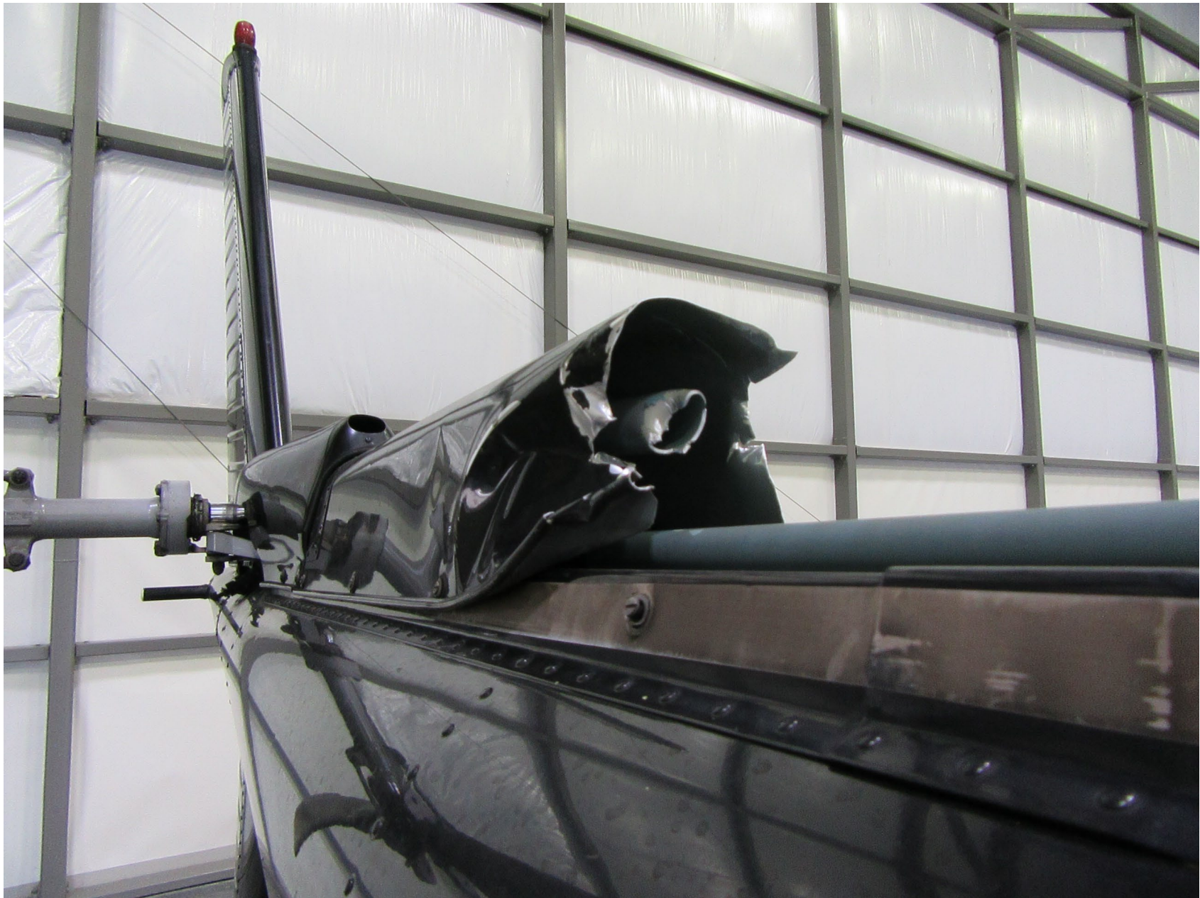
Photo 4 - Fractured Tail Rotor Driveshaft
