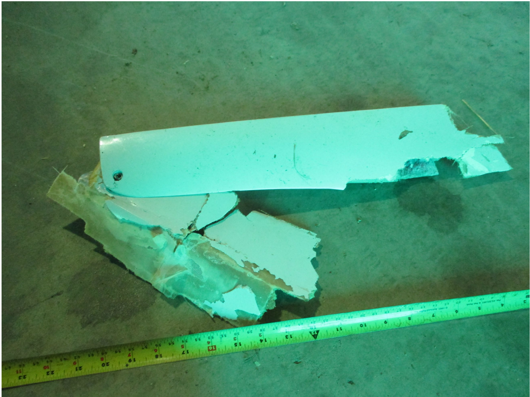
Photo 6 – Left canopy hinge (Photo courtesy of FAA)
