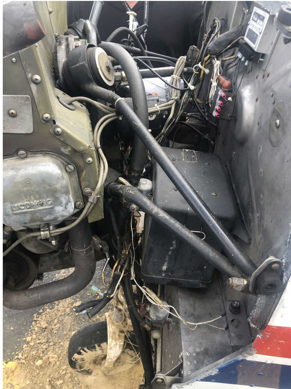
Photo 2 – View of bent engine mount (FAA photo)
