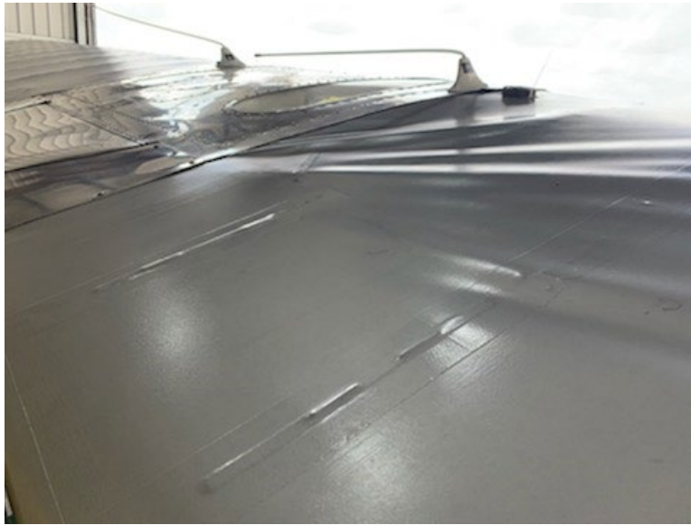
Figure 3: Upper Right Wing Skin Wrinkling
