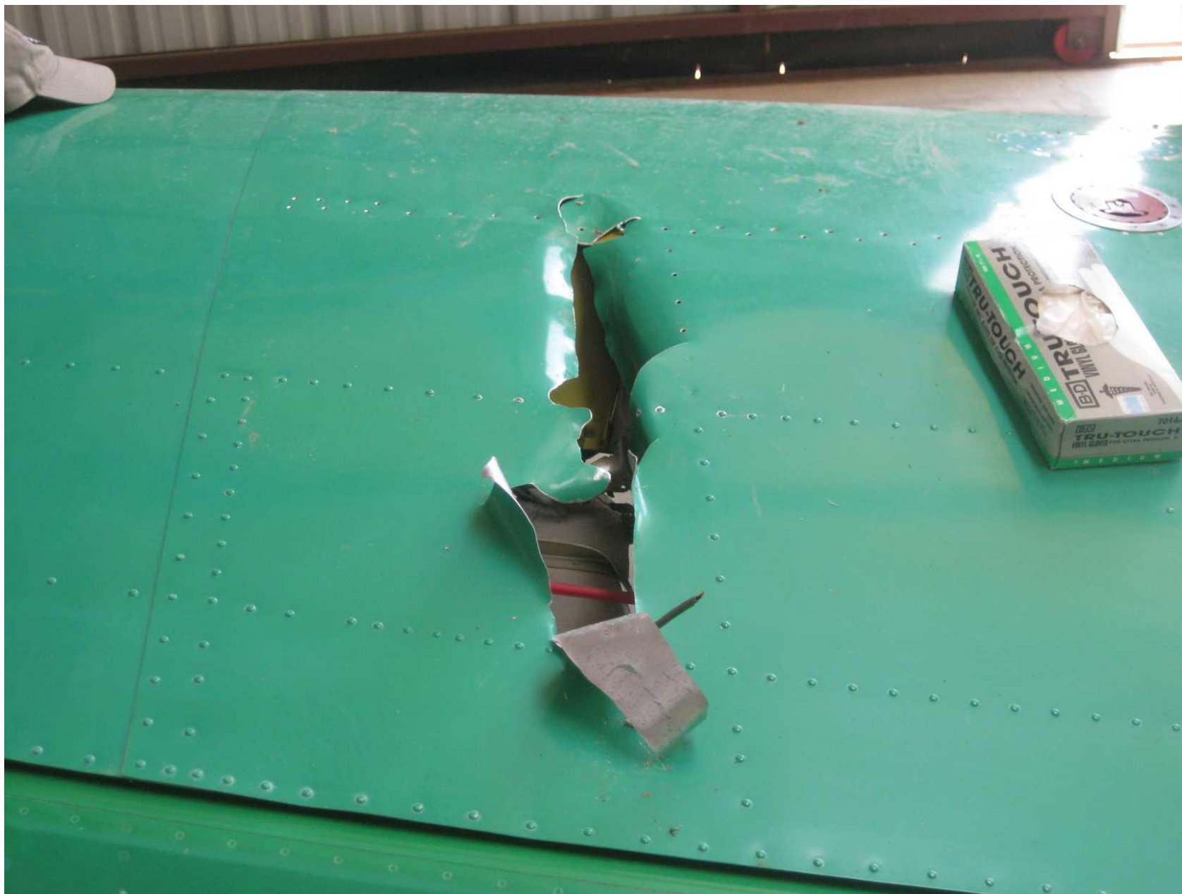
Photo 2 - Left Wing, Top (Photo Provided by Federal Aviation Administration)
