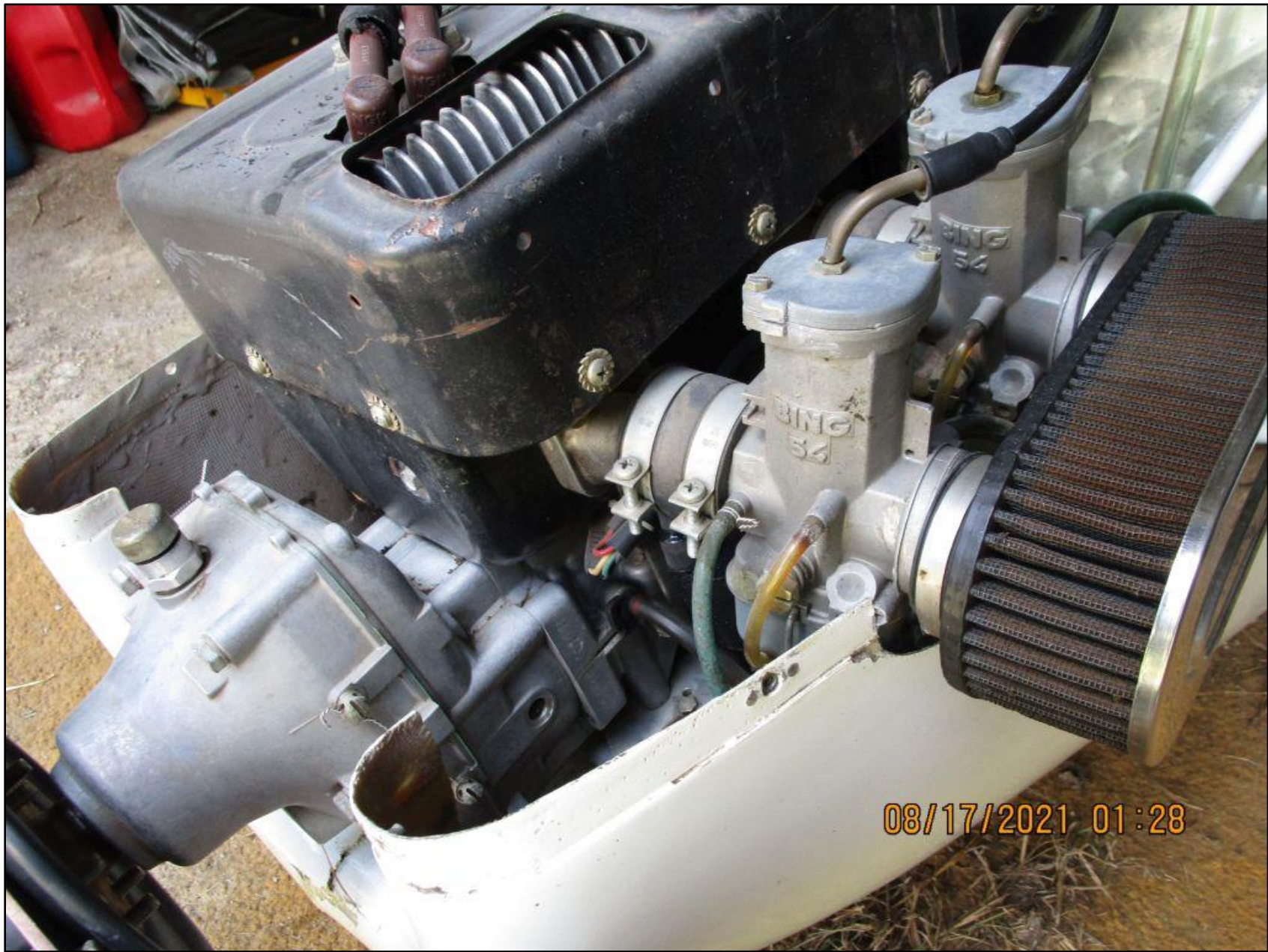
Photo 4 – Engine (FAA Photo)
