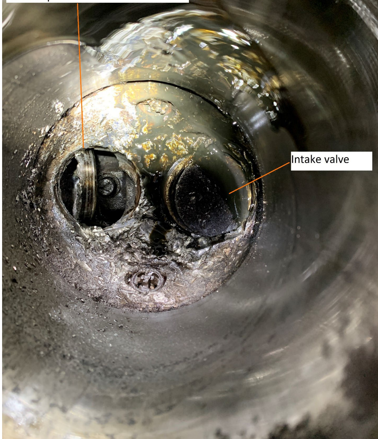
Photo 2: Exhaust Valve (Source – Federal Aviation Administration)
