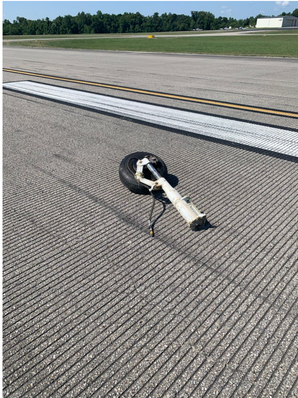
Photo 3 – Separated Landing Gear (FAA Photo)
