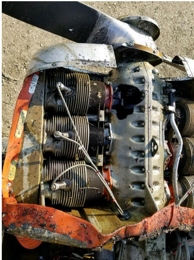
Photo 4: Engine (Photo courtesy of the FAA)
