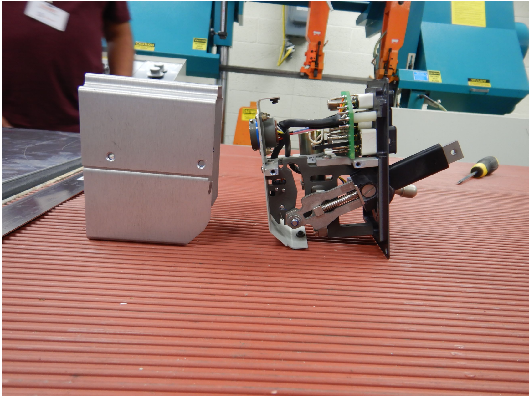
Photo 5 – Inside of landing gear handle
