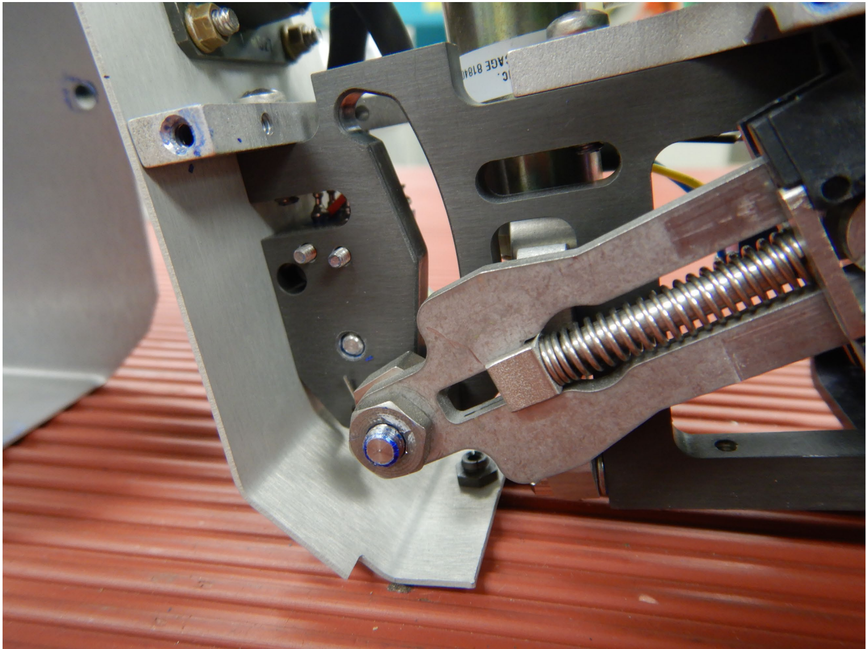
Photo 7 – Landing gear handle, retracted position
