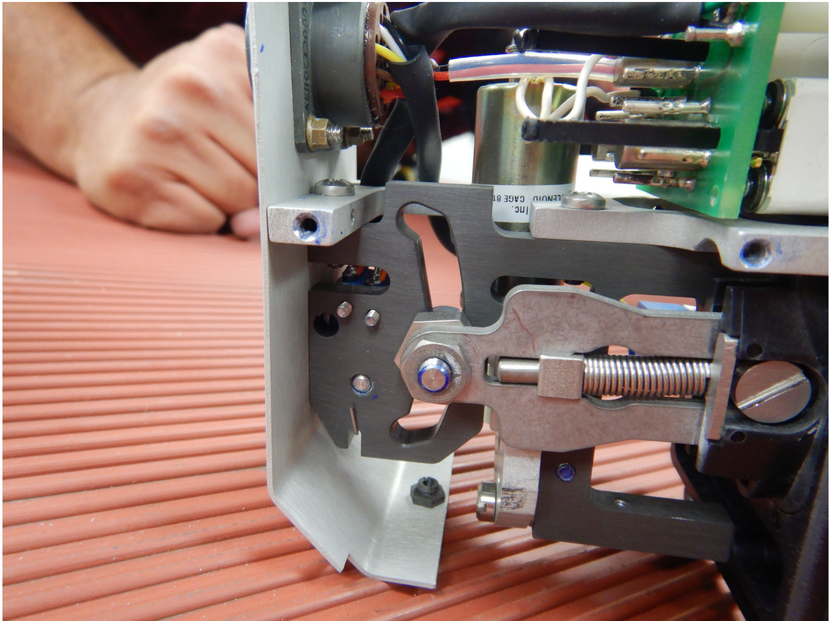
Photo 6 – Landing gear handle, mid travel position
