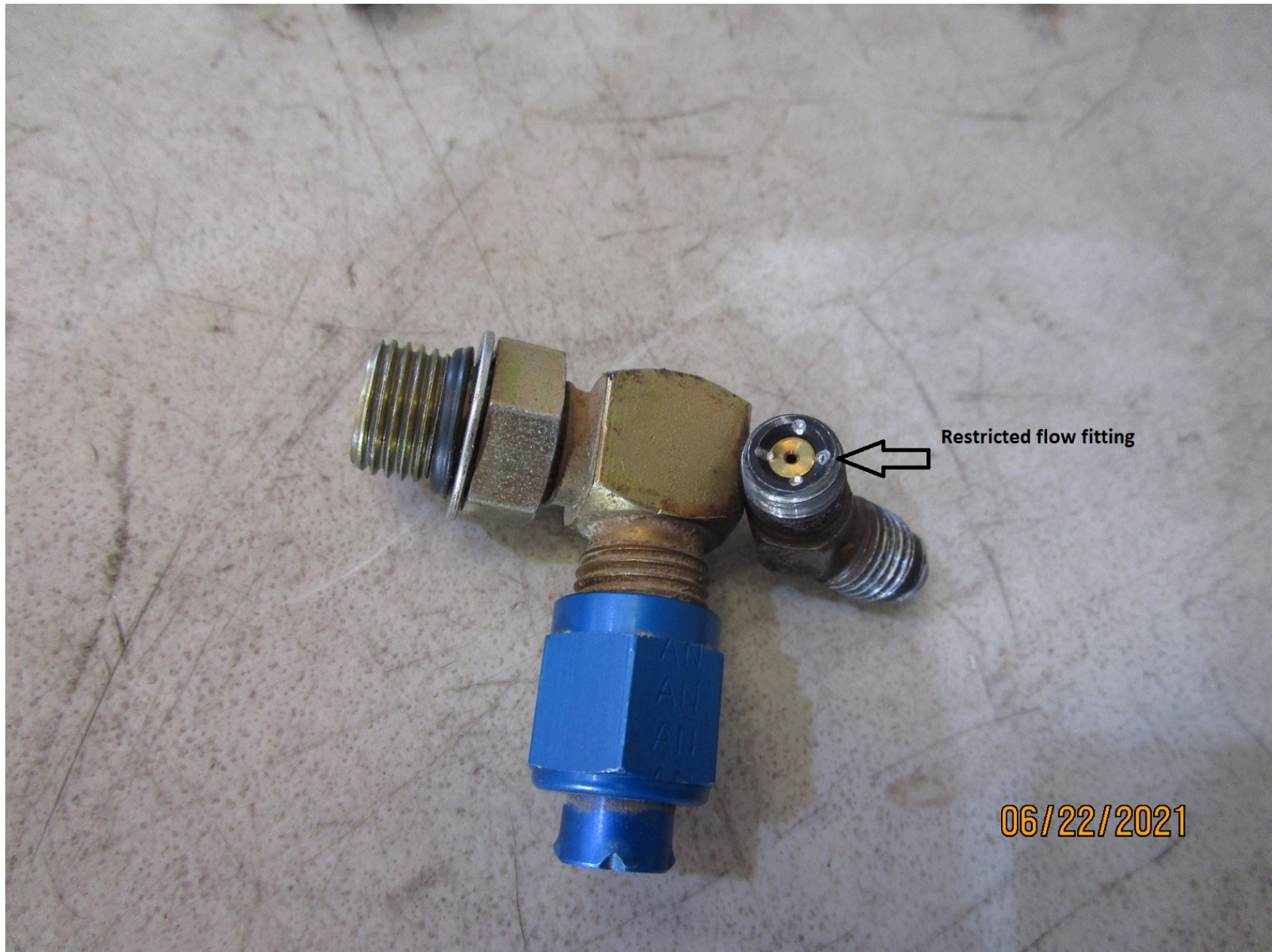
Photo 6 – Fuel pump fitting
