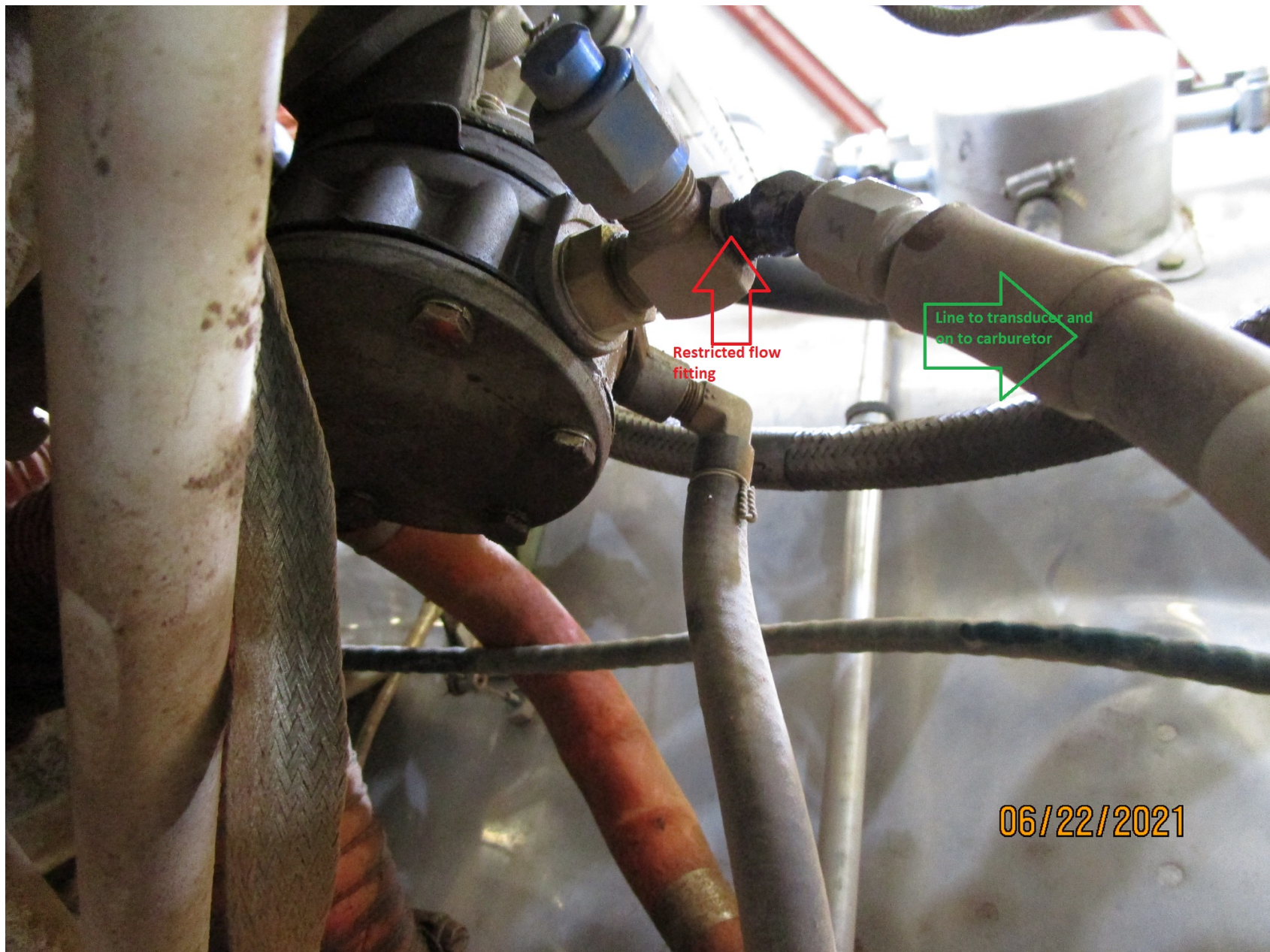
Photo 4 – Engine driven fuel pump
