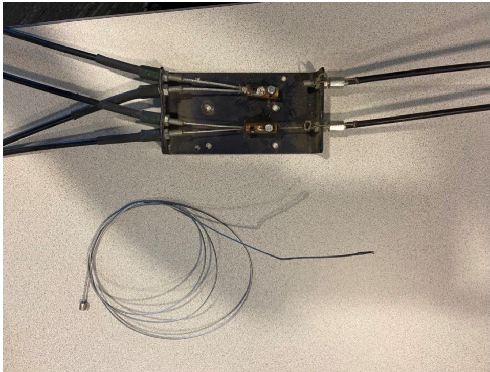
Figure 1: Throttle/Choke Assembly
