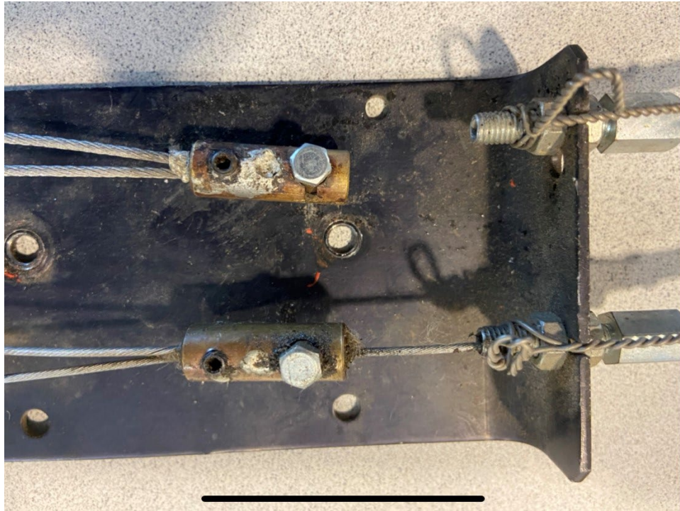
Figure 2: Close View of Throttle/Choke Assembly
