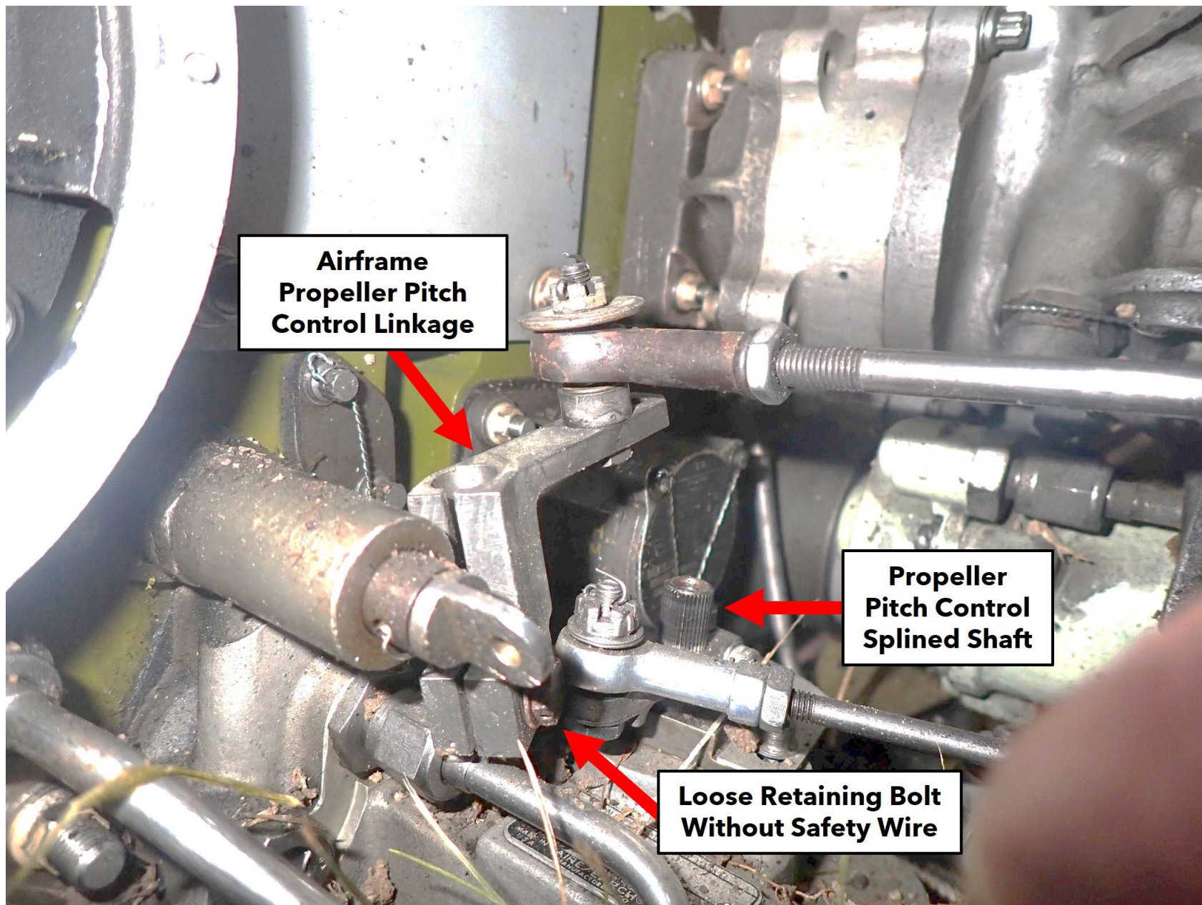
Photo 6 - Airframe Propeller Pitch Control (PPC) Linkage Disconnected from PPC Splined Shaft (Honeywell Aerospace Photo)
