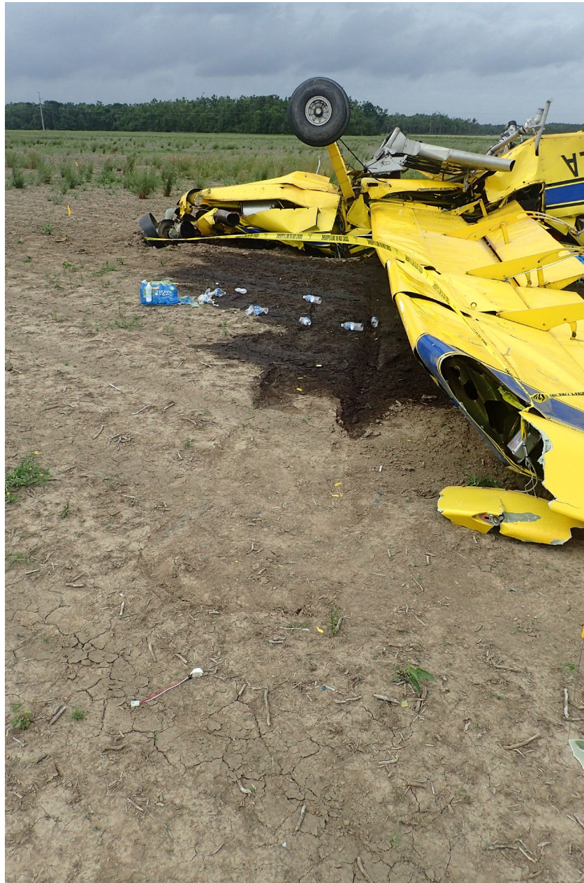
Photo 5 – Right wing (Courtesy of Air Tractor)
