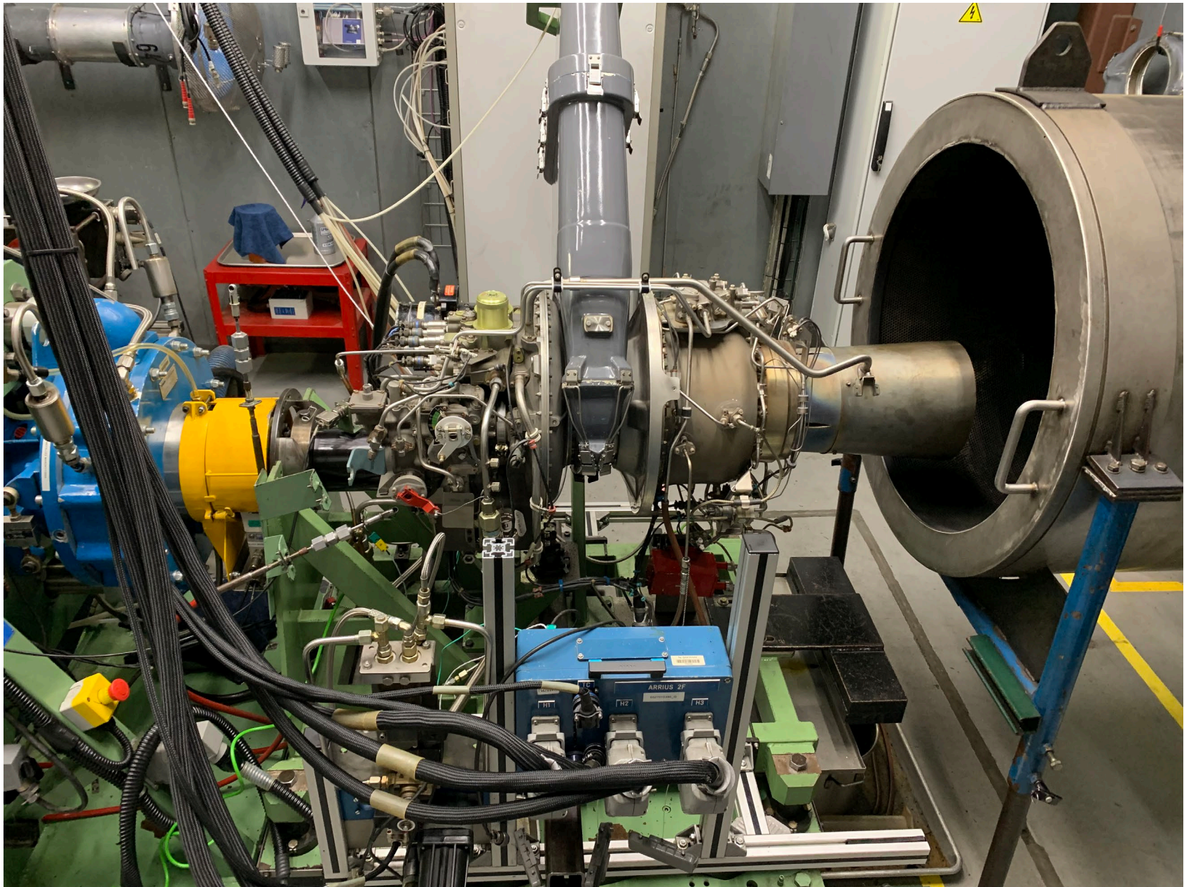
Photo 5 - Engine Mounted in Test Cell (NTSB Photo)
