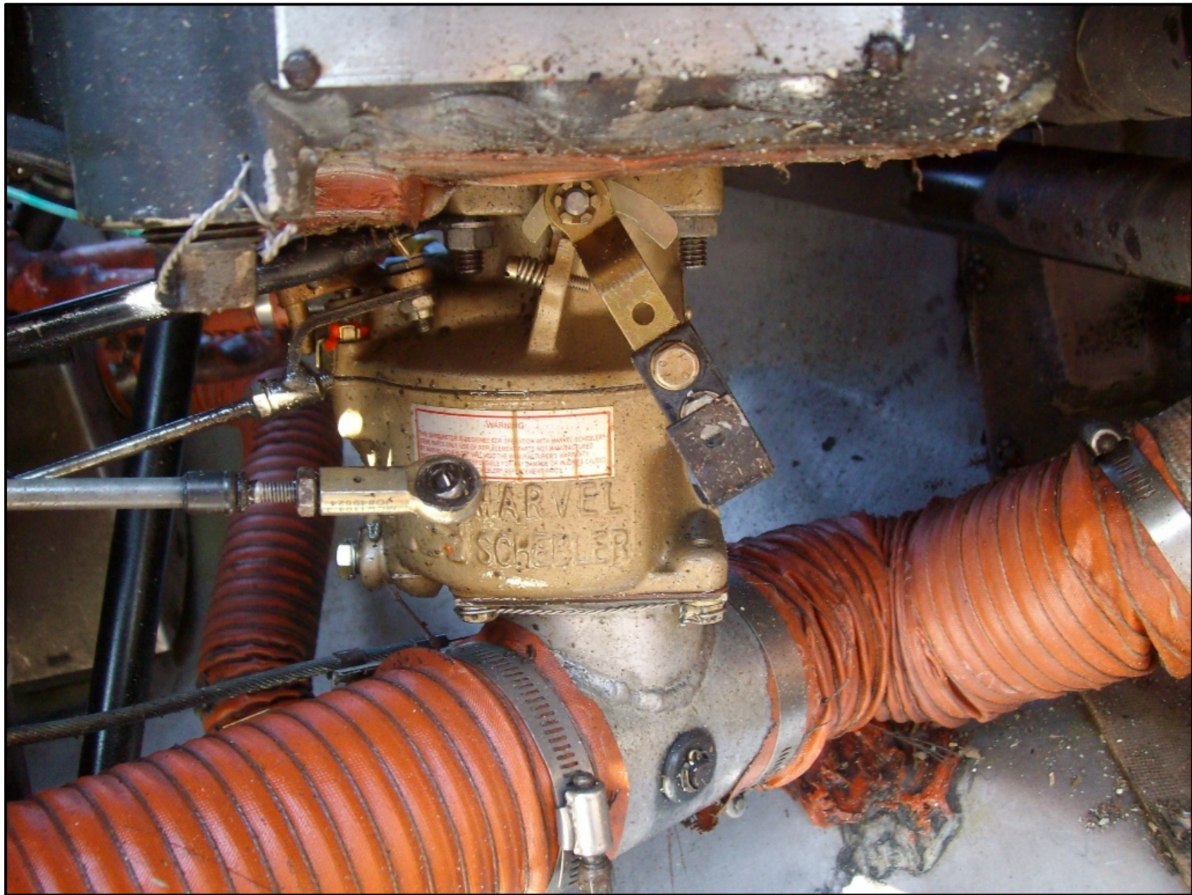
Photo 4 – Carburetor (FAA Photo)
